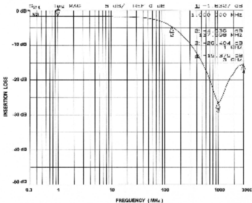
Figure 4. Insertion Loss vs. Frequency Performance Curve, PACUSB-D3(SOT23-6)
