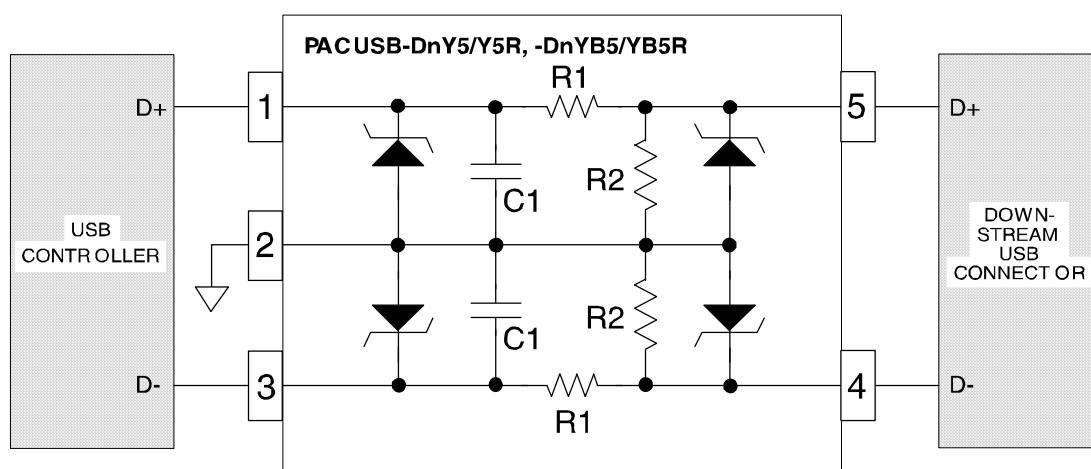
Figure 5. Connection Diagram for PACUSB-D1/D2/D3 Devices
