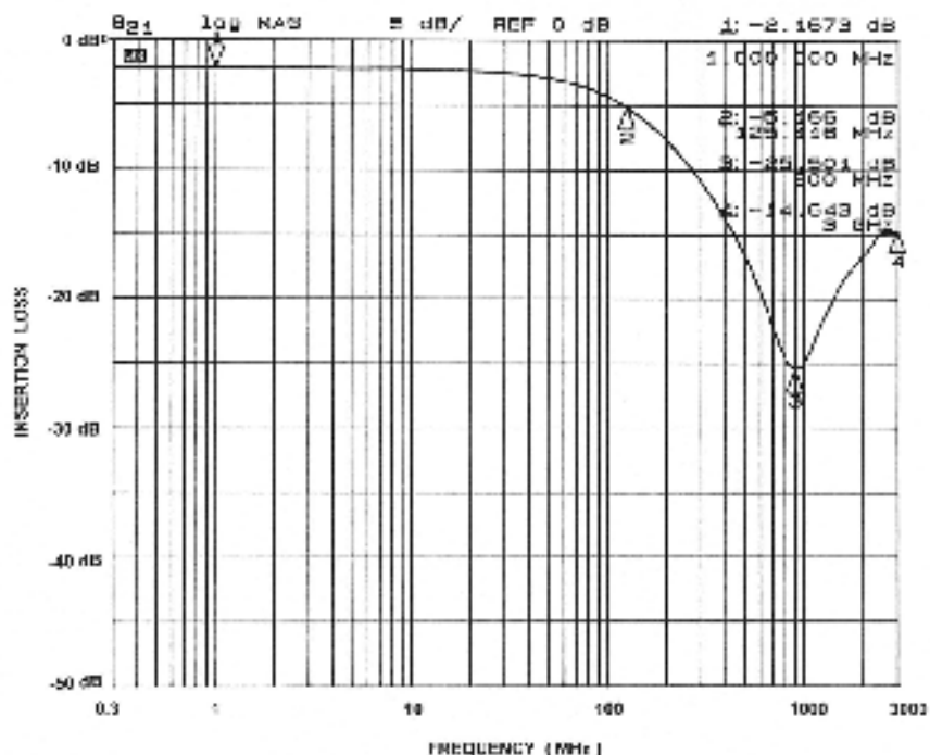
Figure 2. Insertion Loss vs. Frequency Performance Curve, PACUSB-D1(SOT23-6)
