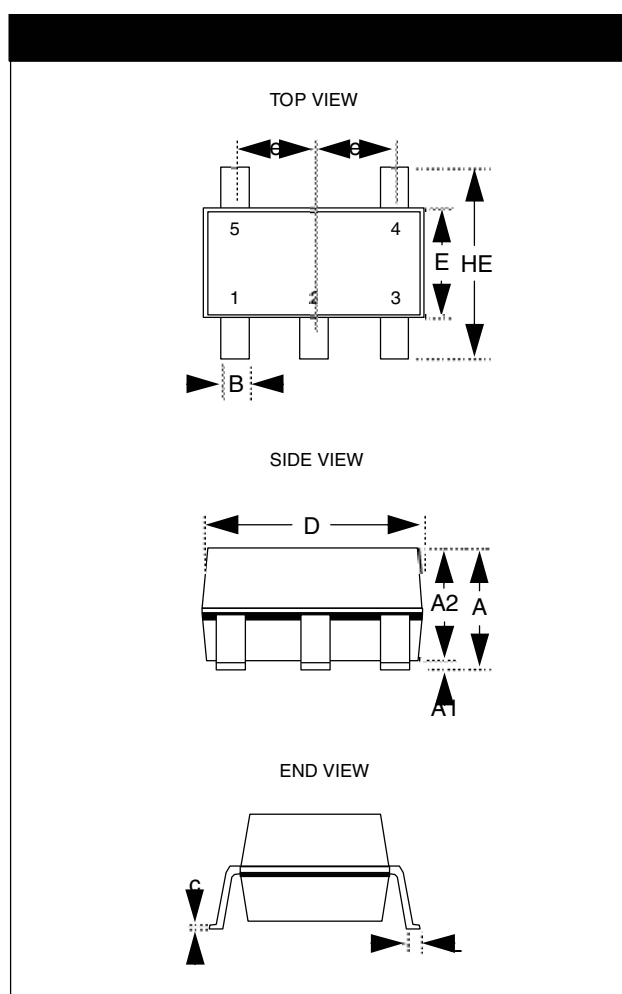
Package Dimensions for SC70-5.
