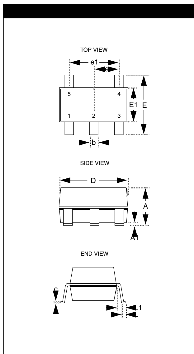
Package Dimensions for SOT23-5.
