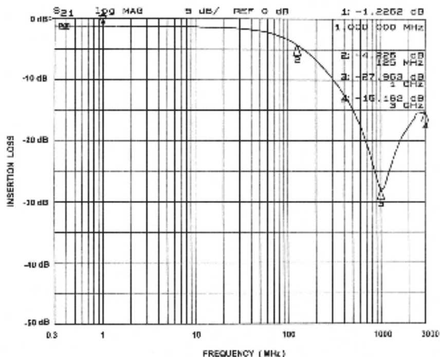
Figure 3. Insertion Loss vs. Frequency Performance Curve, PACUSB-D2(SOT23-
