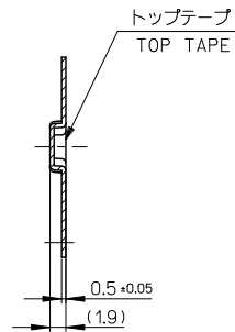
SECT. Y-Y
