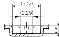
SECT. X-X
