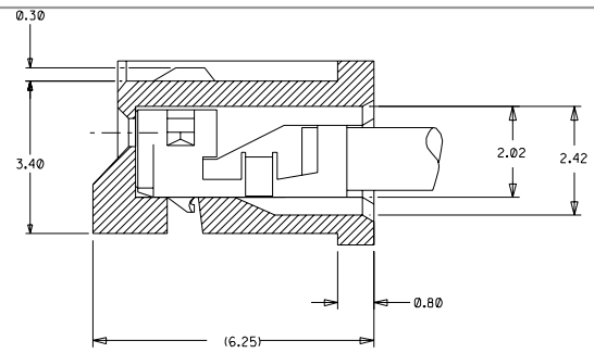
TERMINAL ASSEMBLY DRAWING
