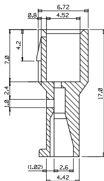
SECTION E-E
