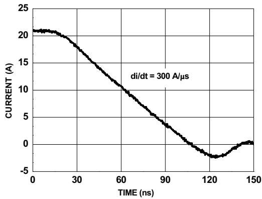
Figure 14. FDMS0308CS SyncFET body diode reverse recovery characteristic
