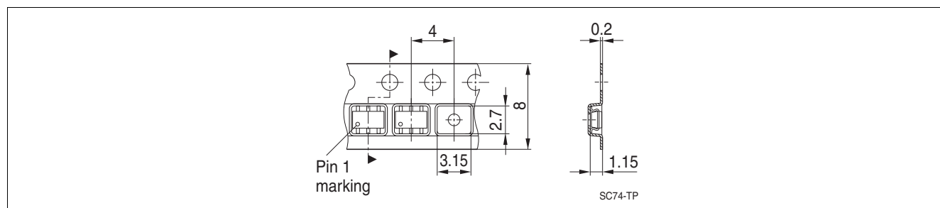
Figure 9 Tape Loading
