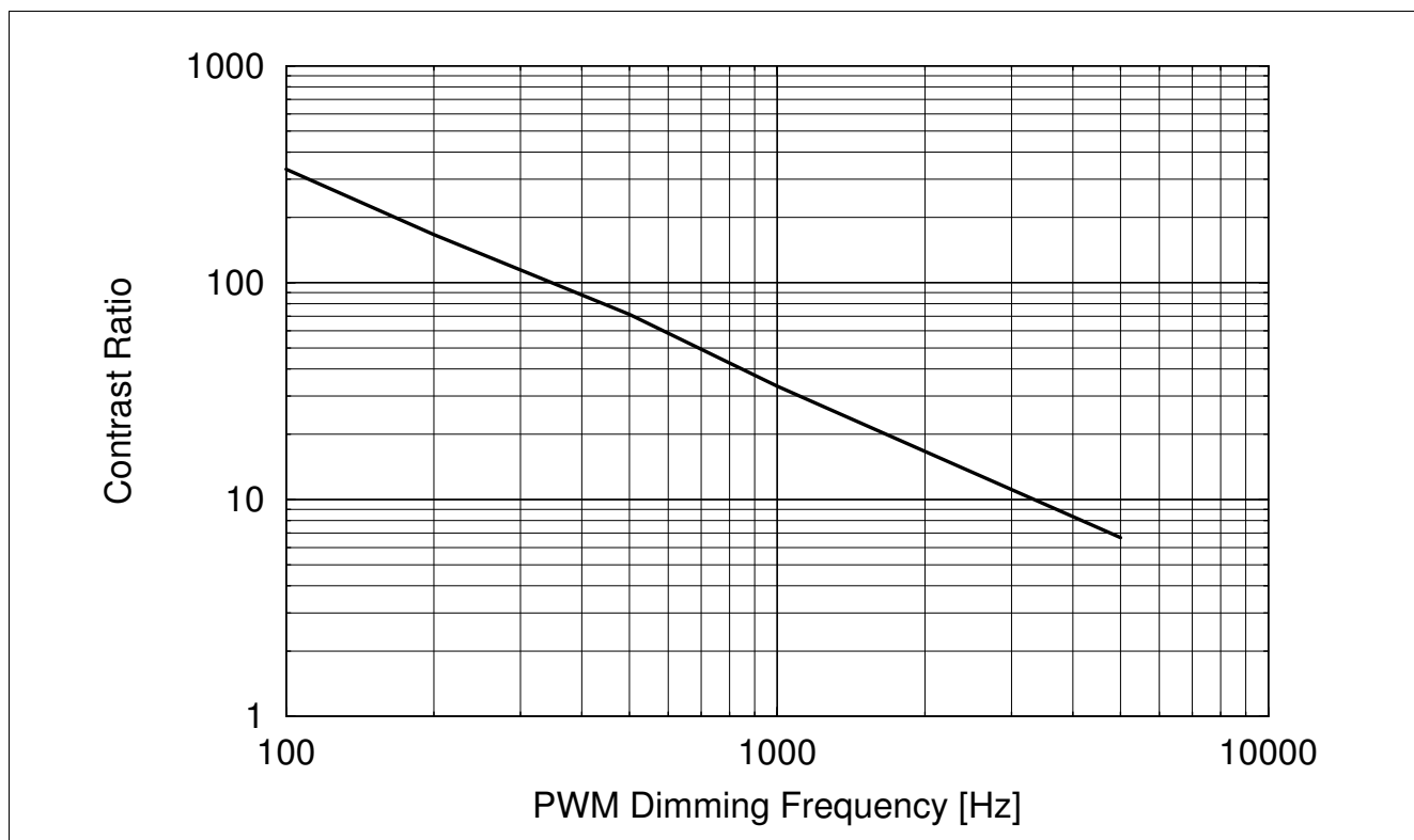
Figure 4 PWM Dimming
