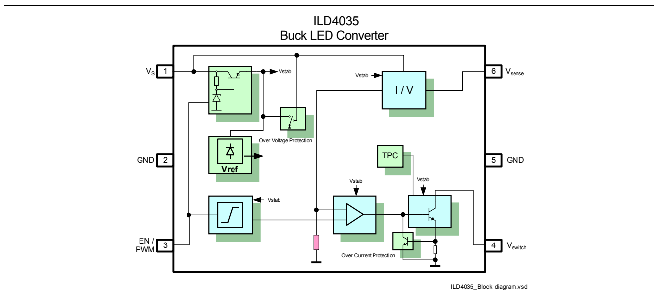
Figure 1 Block Diagram
