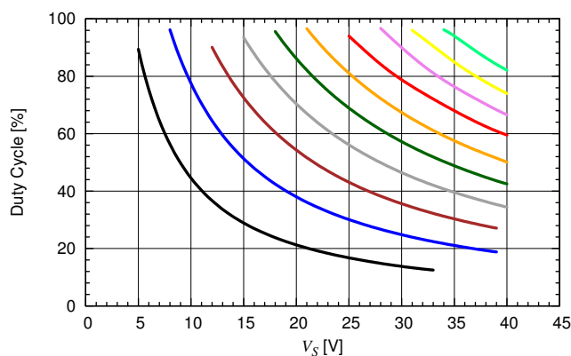
Duty Cycle versus V_S and Number of LEDs
