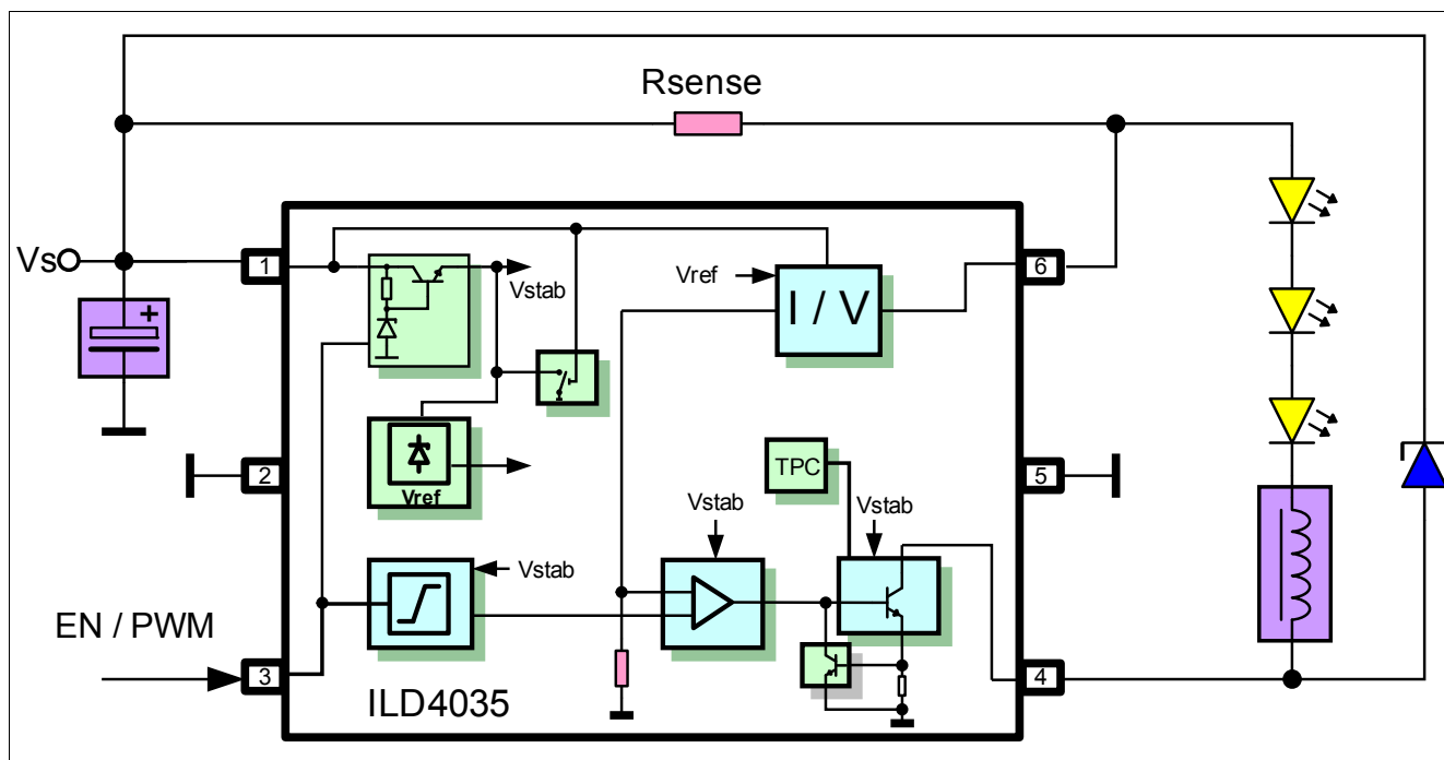
Figure 5 Application Circuit
