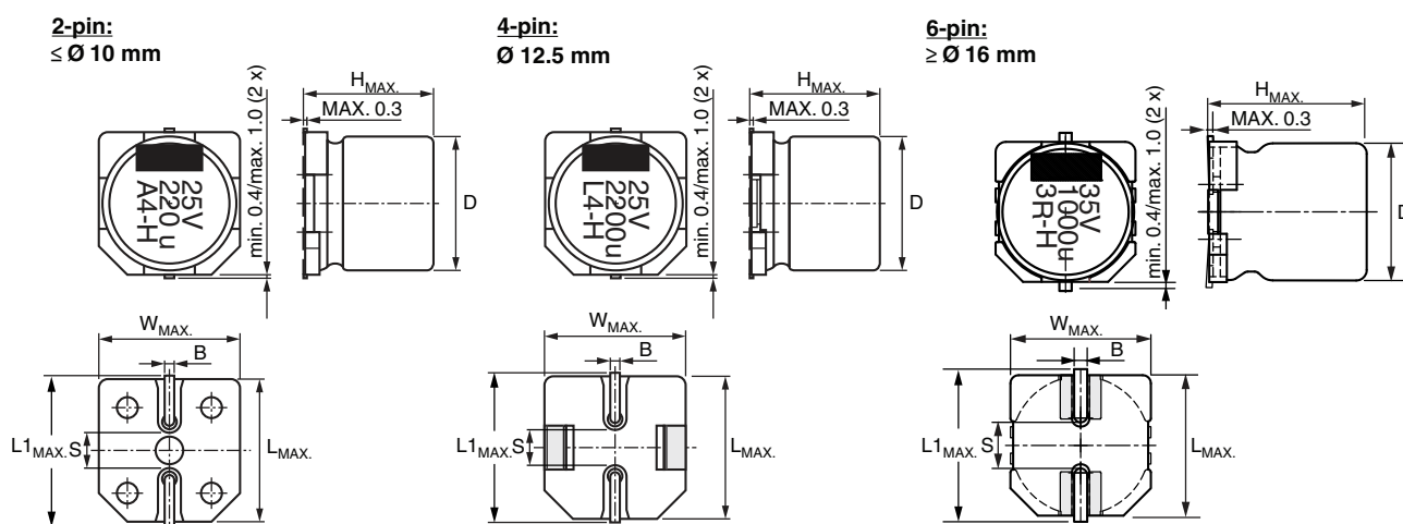
Fig. 2 - Dimensional outline
