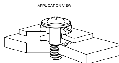
APPLICATION VIEW
