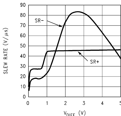
Figure 27. Slew Rate vs. V DIFF
