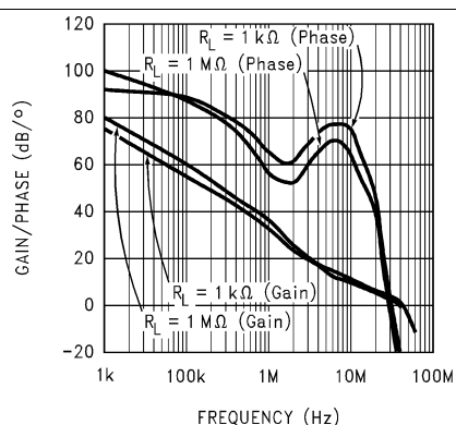
Figure 19. Open Loop Gain/Phase ( V_S = 5V )
