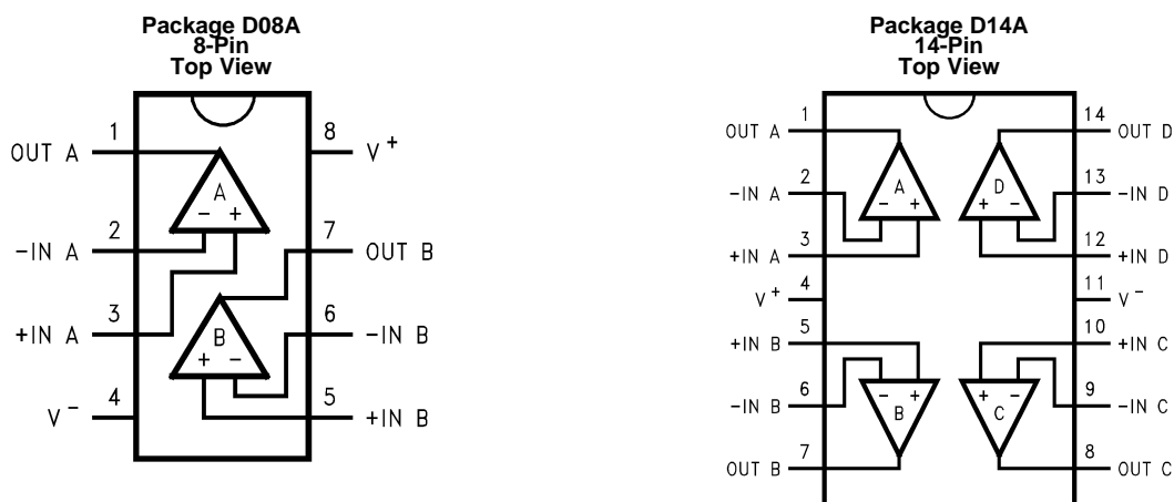
Pin Functions
