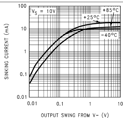
Figure 10. Output Voltage vs. Sink Current
