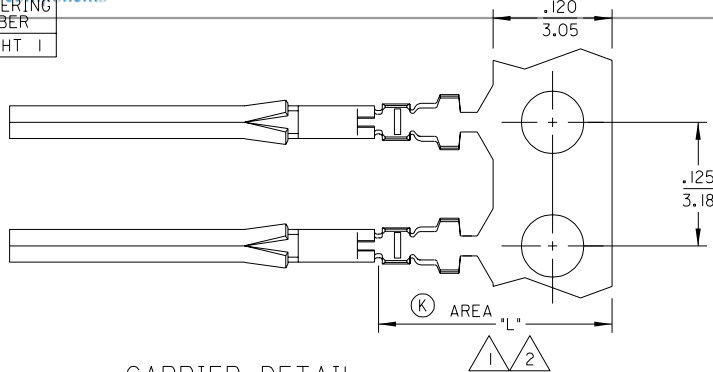
CARRIER DETAIL
