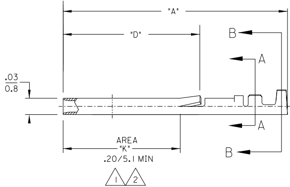
CARRIER DETAIL
