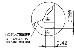
DETAIL A (SCALE 20:1)
