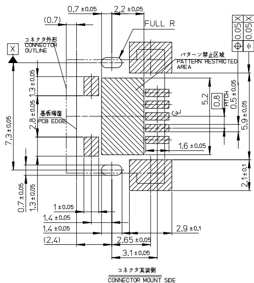
推薦基板寸法 (SCALE 8:1) RECOMMENDED PCB PATTERN LAYOUT
