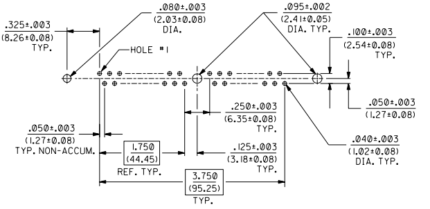
RECOMMENDED SOCKET P.C. BOARD HOLE PATTERN
