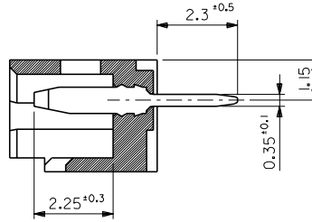
SECT. X-X
