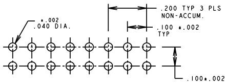
RECOMMENDED P.C. BOARD HOLE PATTERN
