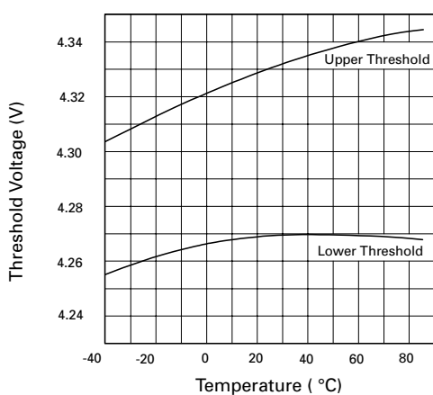
Threshold Voltage vs. Temperature
