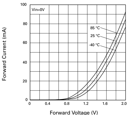
Clamp Diode Forward Current vs. Voltage
