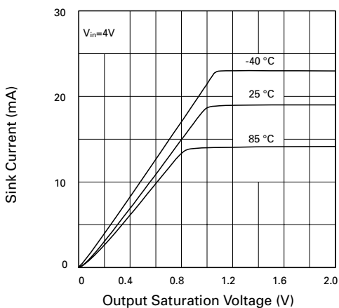
Output Saturation Voltage vs. Sink Current
