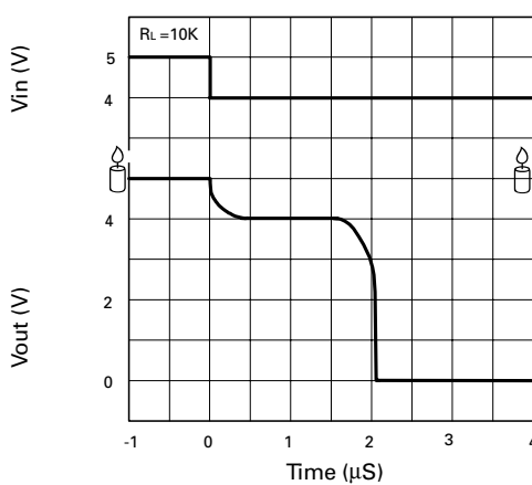
Reset Delay Time
