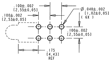
RECOMMENDED HOLE PATTERN GAUGE
