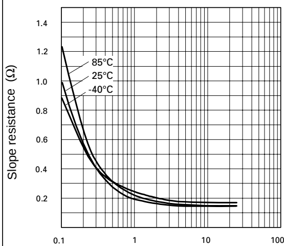
Reference Current (mA) Slope Resistance v Current
