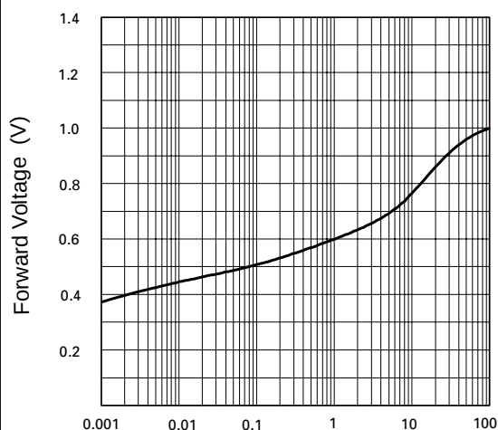
Forward Current (mA) Forward Characteristics
