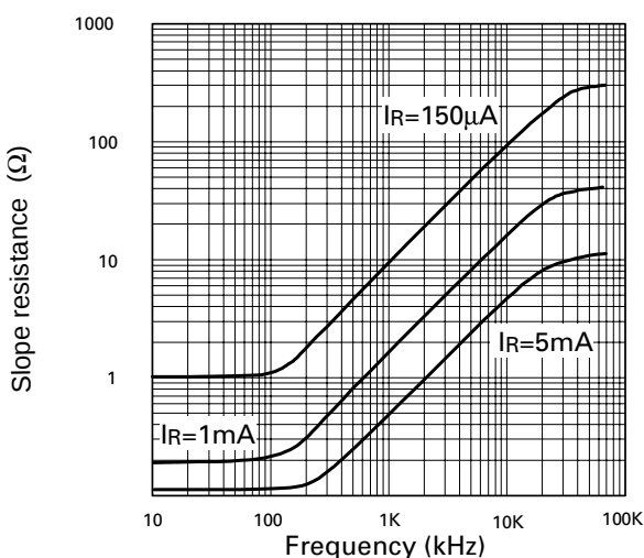
Frequency (kHz) Slope Resistance v Frequency
