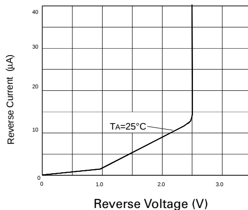
Reverse Characteristics
