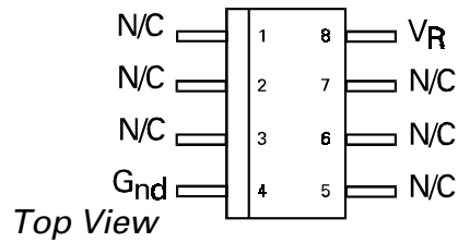
SO8 Package Suffix - N8
