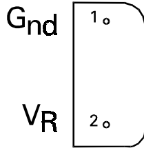
E-Line, 2 pin Package Suffix - Y
