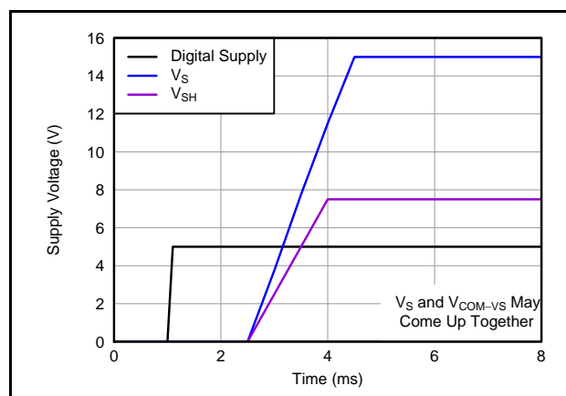
Figure 20. Startup Requirement with Two Supplies
