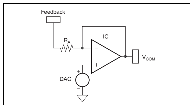
Figure 27. Configuration for Switch Position 8
