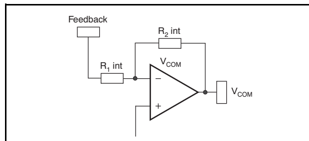
Figure 26. Configuration for Switch Positions 2, 3, 4, 5, 6, 7
