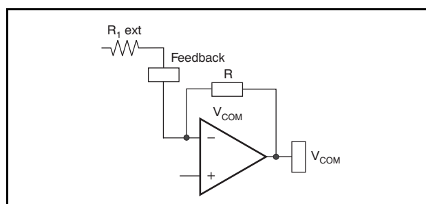
Figure 28. Configuration for Switch Position 1
