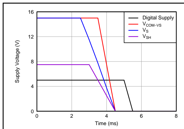
Figure 23. Shutdown Requirement with Three Supplies
