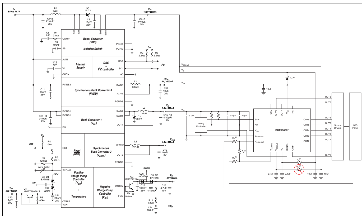
Figure 24. Typical Application Circuit using the TPS65168
