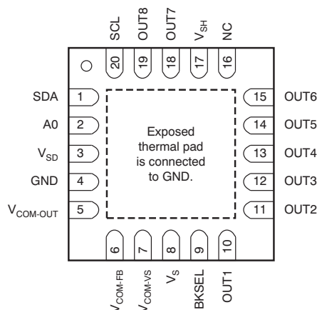
RGW PACKAGE VQFN-20 (TOP VIEW)
