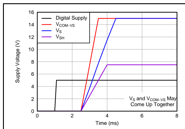
Figure 21. Startup Requirement with Three Supplies
