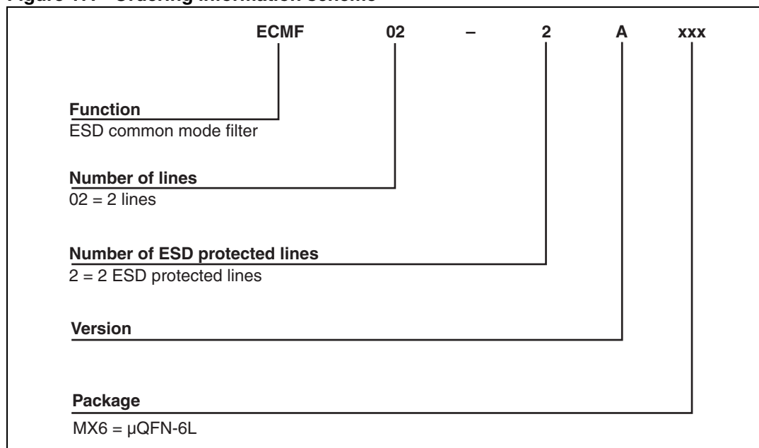
Figure 17. Ordering information scheme
