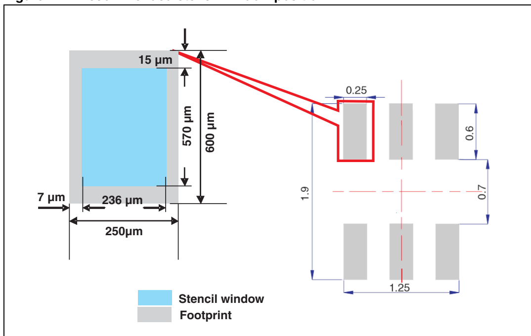
Figure 22. Recommended stencil window position
