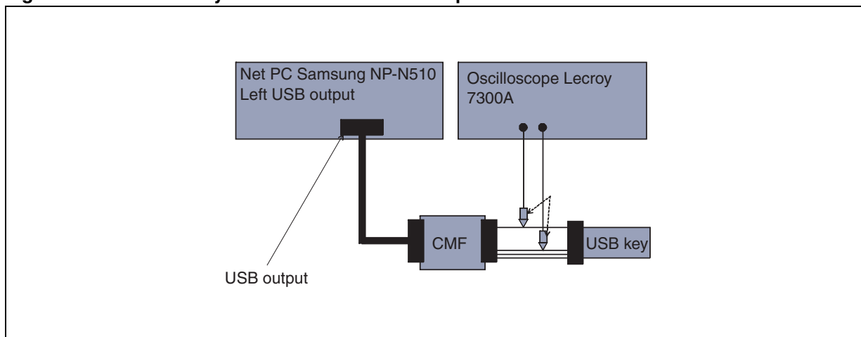
Figure 12. USB 2.0 HSync measurement test setup
