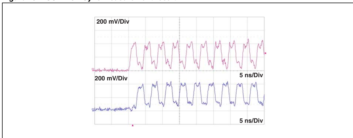
Figure 13. USB 2.0 HSync measurement result
