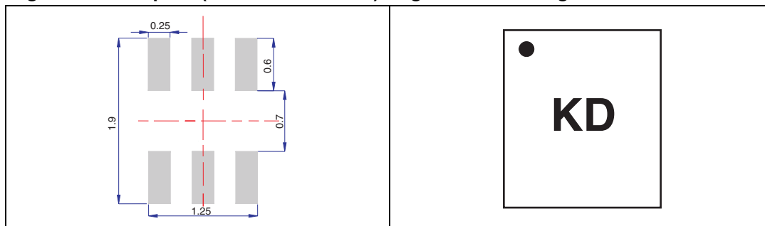
Figure 18. Footprint (dimensions in mm) Figure 19. Marking
