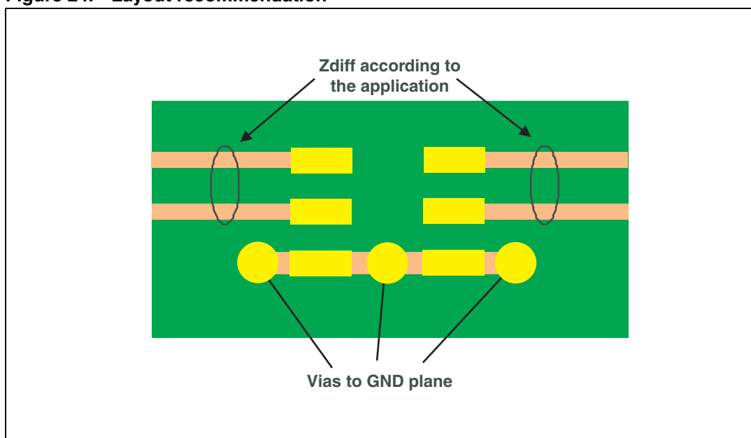
Figure 24. Layout recommendation
