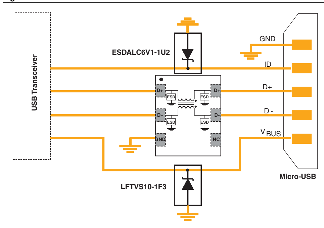
Figure 16. USB 2.0
