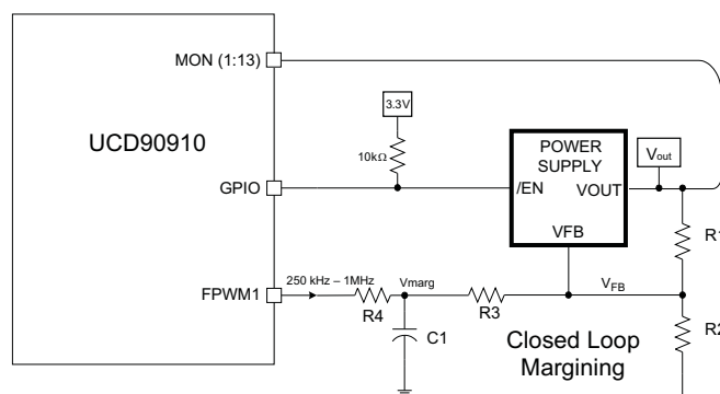
Figure 20. Closed-Loop Margining
