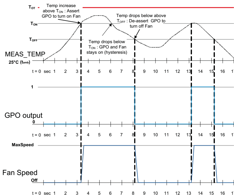
Figure 24. Hysteretic Temperature Control for 2- or 3-Wire Fans
