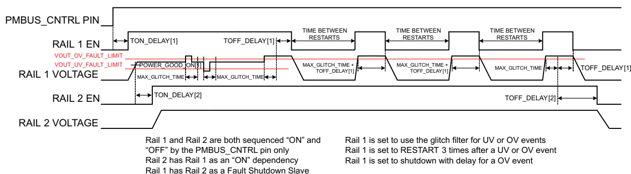
Figure 13. Sequencing and Fault-Response Timing
