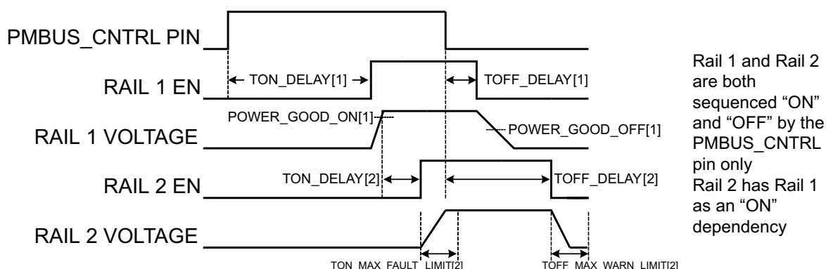
Figure 8. Sequence-on and Sequence-off Timing
