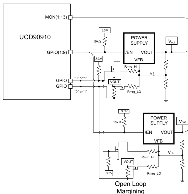
Figure 19. Open-Loop Margining
