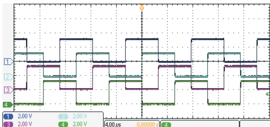
Figure 18. Multiphase PWMs
