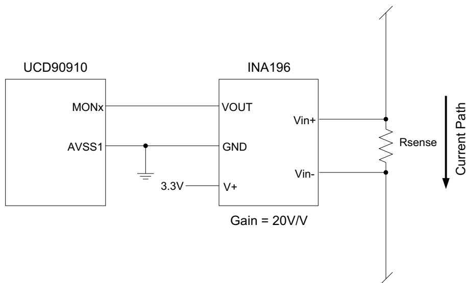
Figure 10. Current Monitoring Circuit Example Using the INA196
