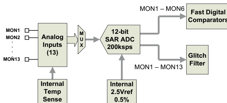
Figure 9. Monitoring Block Diagram
