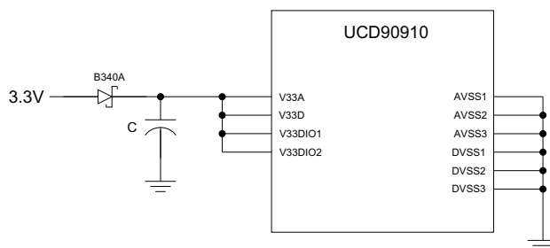
Figure 28. Brownout Circuit
