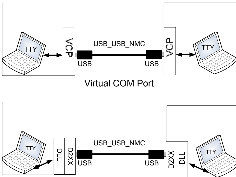
Figure 1.1 USB to USB Null Modem Cable Example
