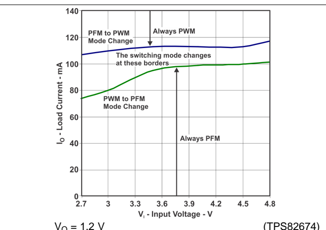
Figure 40. PFM/PWM Boundaries
