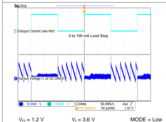
Figure 31. Load Transient Response in PFM/PWM Operation
