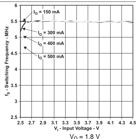
Figure 2. PWM Switching Frequency vs. Input Voltage
