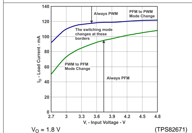
Figure 39. PFM/PWM Boundaries
