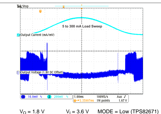
Figure 30. AC Load Transient Response
