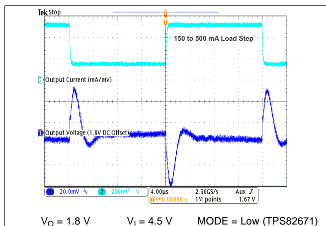
Figure 29. Load Transient Response in PFM/PWM Operation
