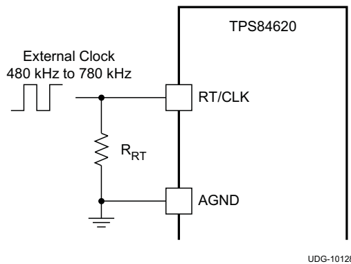
Figure 36. CLK/RT Configuration
