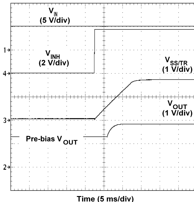
Figure 29. Start-up into Pre-bias
