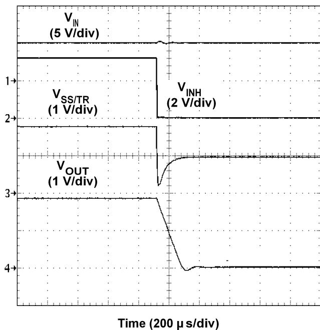
Figure 31. Inhibit Turn-Off
