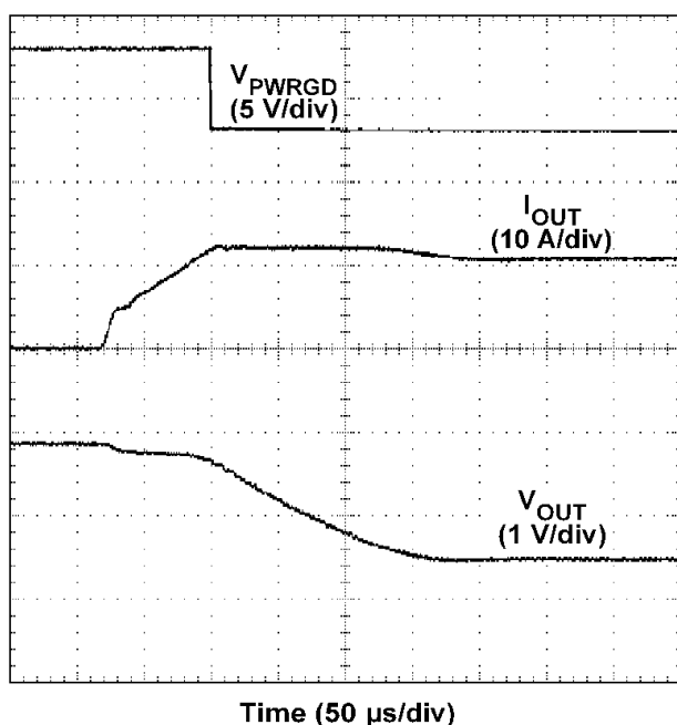
Figure 34. Overcurrent Limiting
