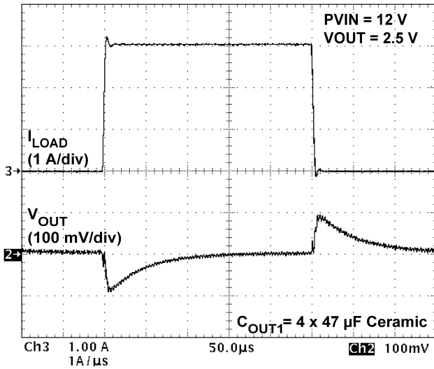
Figure 21. PV_{IN} = 12\text{V} , V_{OUT} = 2.5\text{V} , 3A Load Step
