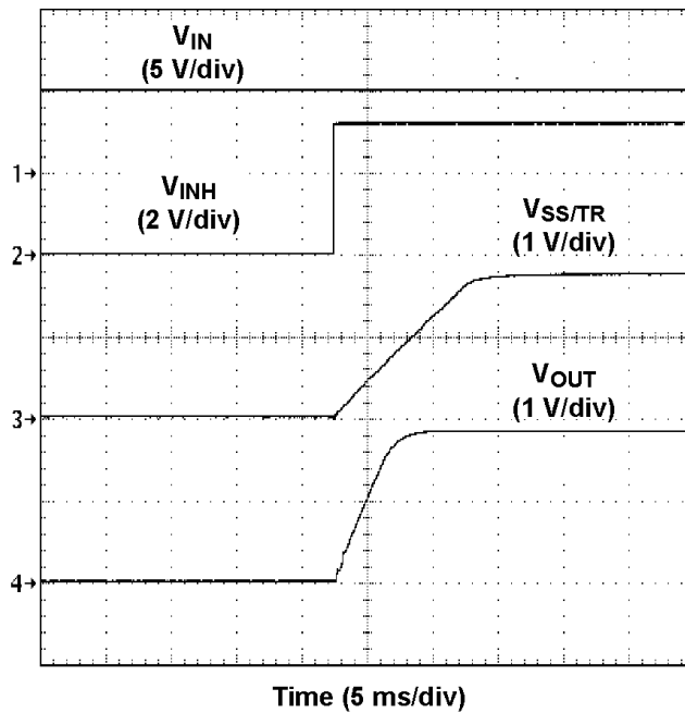
Figure 32. Inhibit Turn-On
