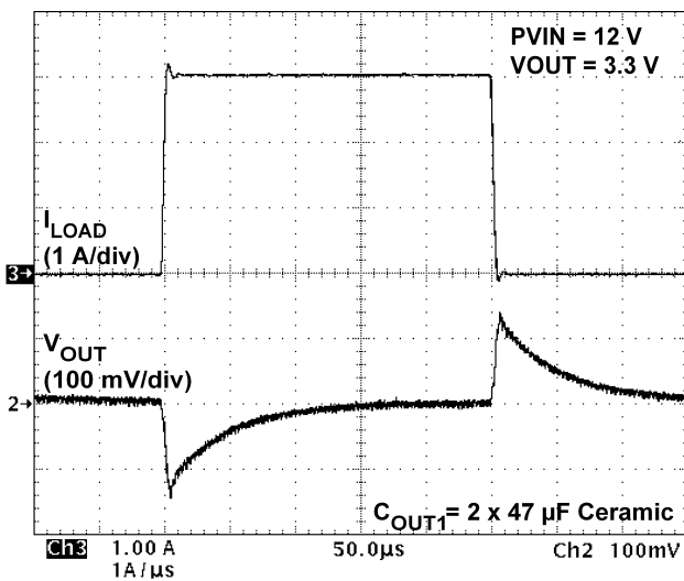
Figure 23. PV_{IN} = 12\text{V} , V_{OUT} = 3.3\text{V} , 3A Load Step
