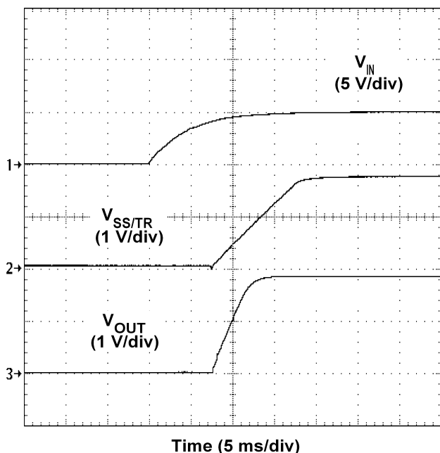
Figure 28. Start-Up Waveforms
