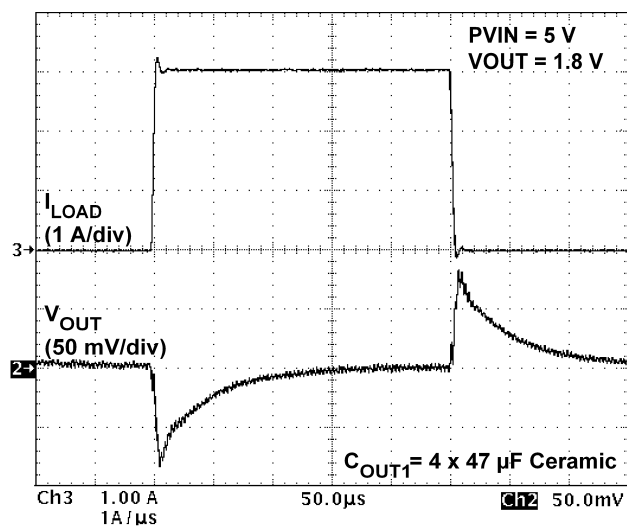
Figure 20. P_{VIN} = 5V , V_{OUT} = 1.8V , 3A Load Step
