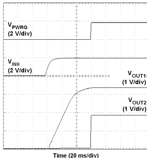
Figure 38. Sequencing Waveforms
