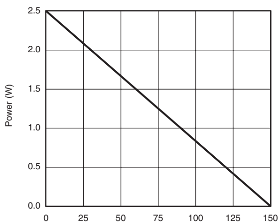
Power, Junction-to-Foot
