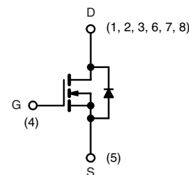
N-Channel MOSFET
