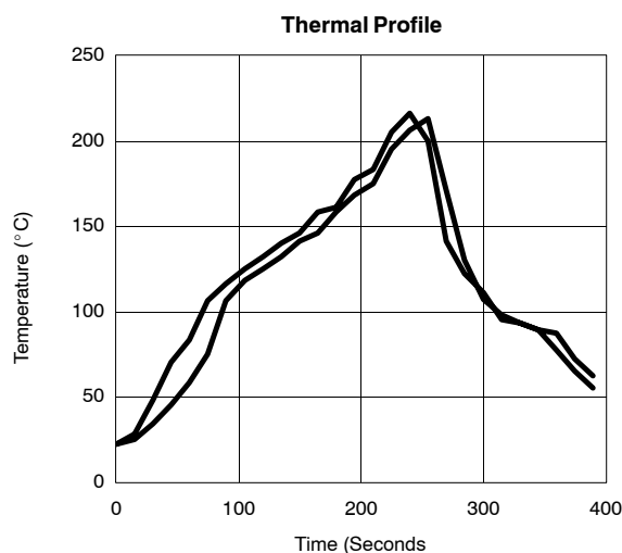
FIGURE 6. Reflow Profile
