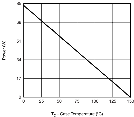
Power, Junction-to-Case
