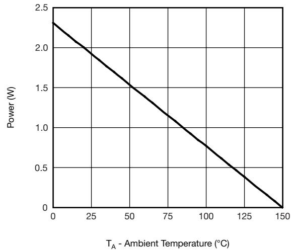
Power, Junction-to-Ambient
