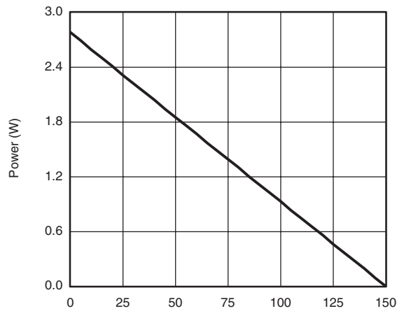
Power, Junction-to-Ambient
