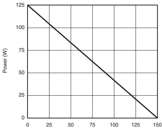
Power, Junction-to-Case
