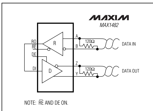
Figure 16. Line Repeater for MAX1482
