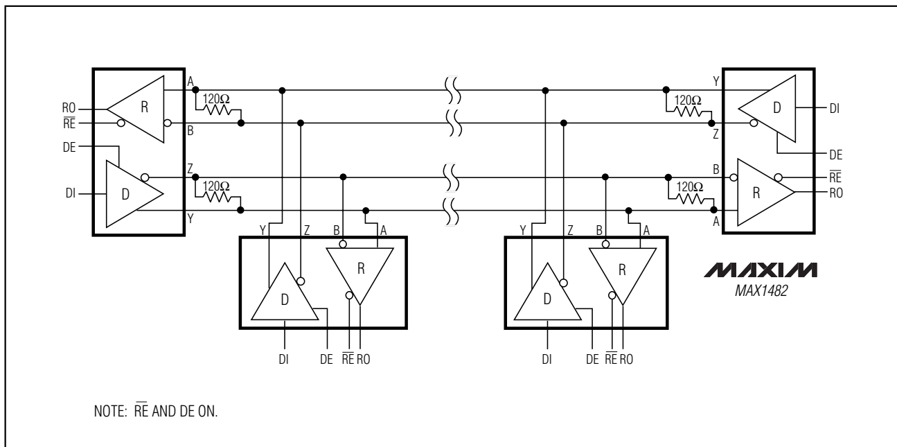
Figure 15. MAX1482 Full-Duplex RS-485 Network
