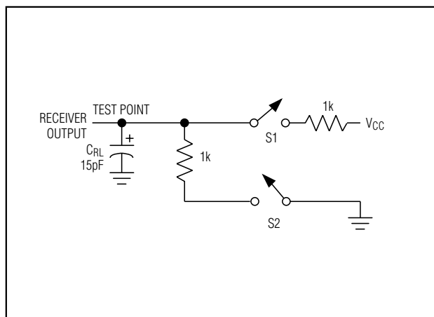
Figure 2. Receiver Timing Test Load
