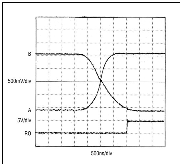
Figure 12. Receiver t_{PLH}
