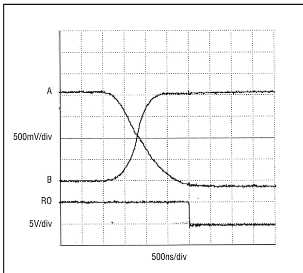
Figure 11. Receiver t_{PHL}
