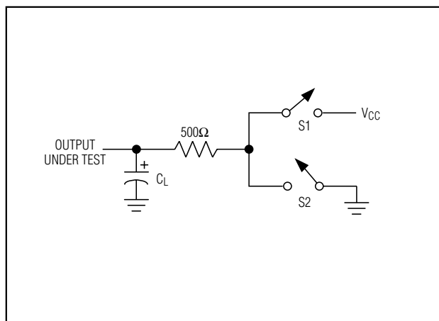
Figure 4. Driver Timing Test Load
