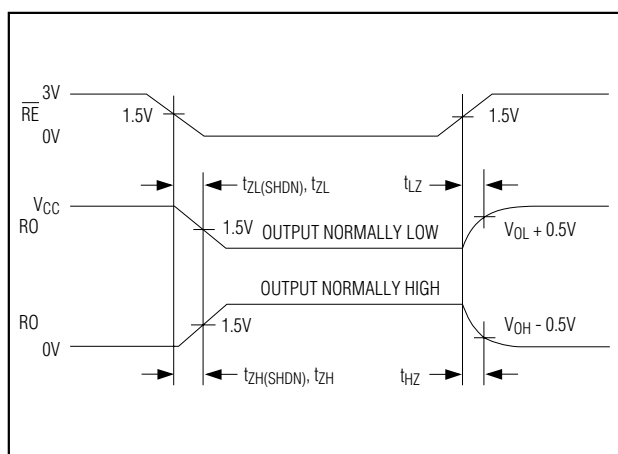
Figure 8. Receiver Enable and Disable Times
