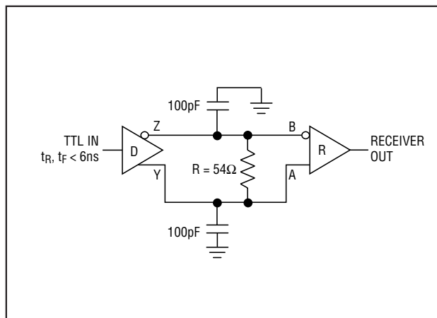
Figure 10. Receiver Propagation-Delay Test Circuit
