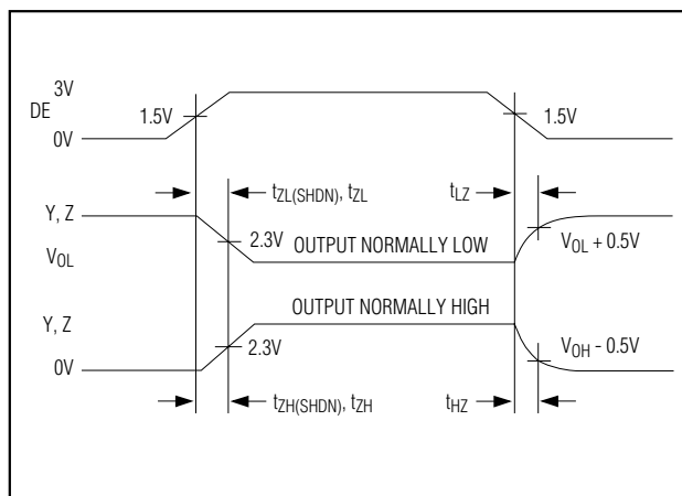
Figure 6. Driver Enable and Disable Times
