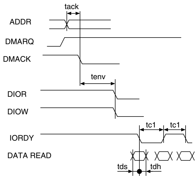
Figure 15. Timing for UDMA In-Transfer Start
