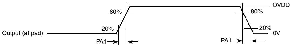
Figure 4. Output Pad Transition Time Waveform
