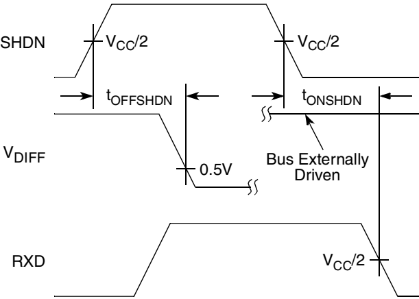
Figure 62. Timing Diagram for FlexCAN Shutdown Signal
