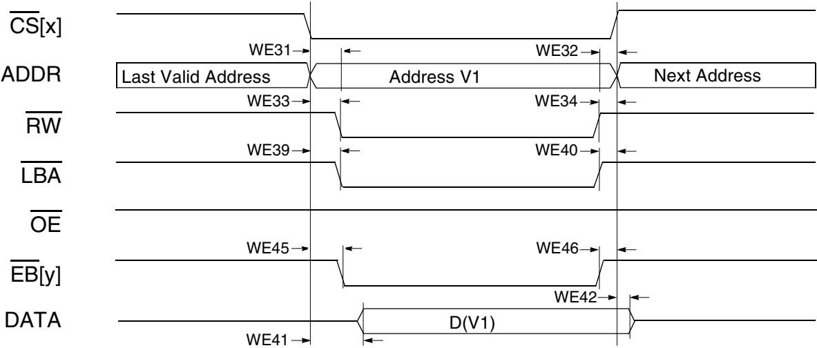
Figure 47. Asynchronous Memory Write Access
