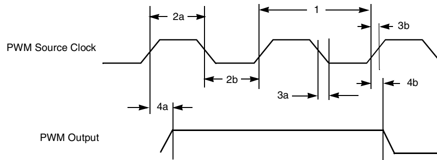
Figure 67. PWM Timing
