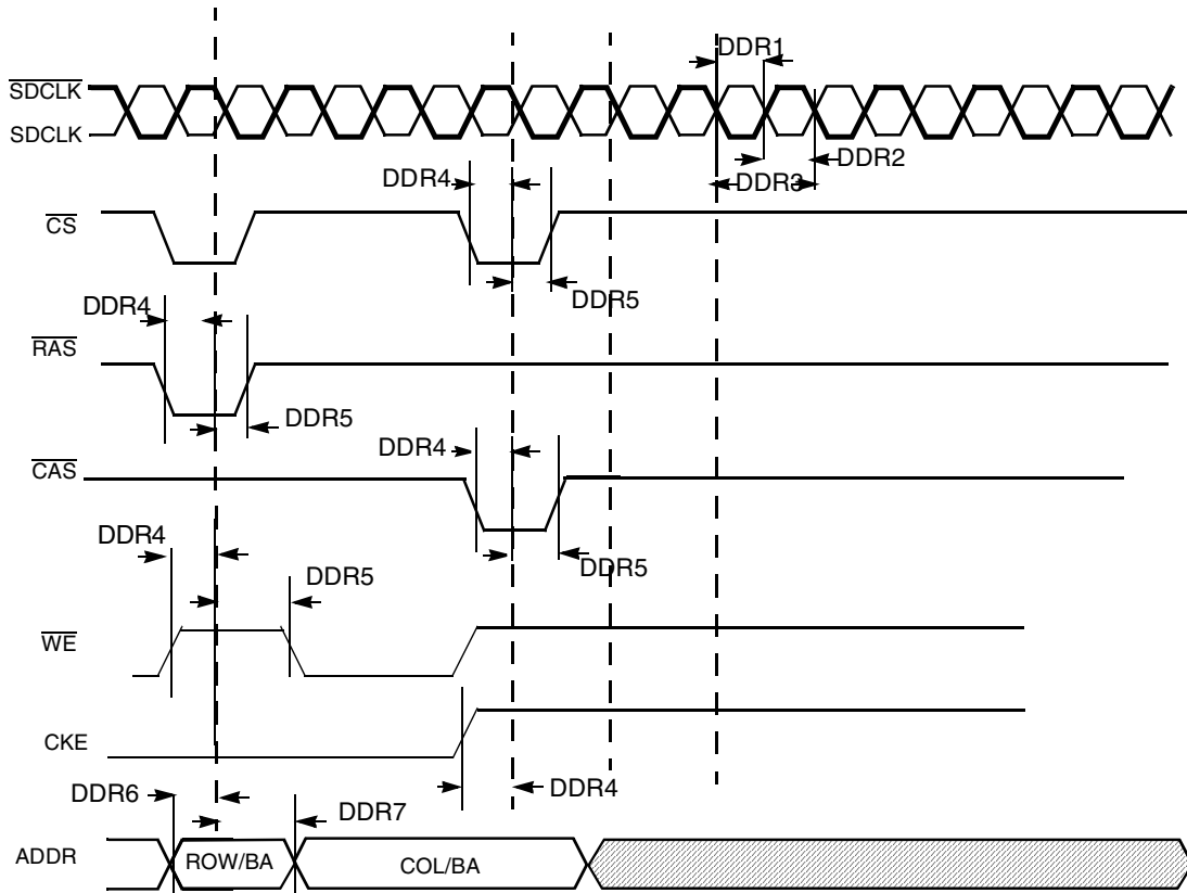
Figure 31. DDR2 SDRAM Basic Timing Parameters
