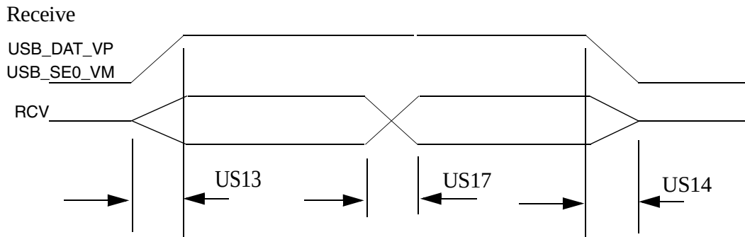
Figure 92. USB Receive Waveform in DAT_SE0 Unidirectional Mode
