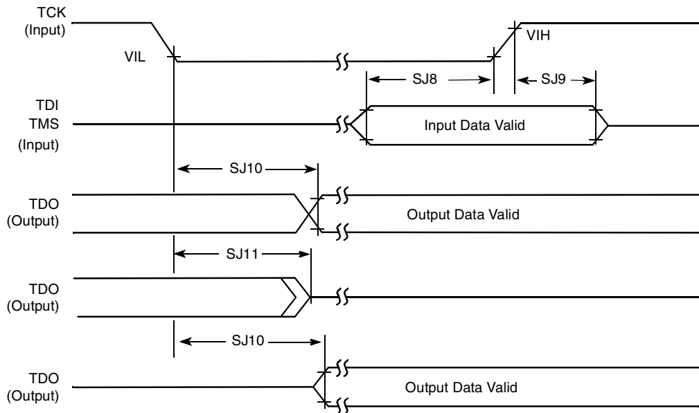
Figure 74. Test Access Port Timing Diagram
