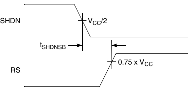
Figure 63. Timing Diagram for FlexCAN Shutdown-to-Standby Signal
