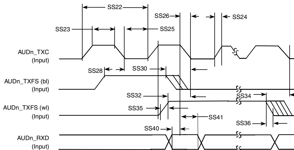
Figure 81. SSI Receiver with External Clock Timing Diagram
