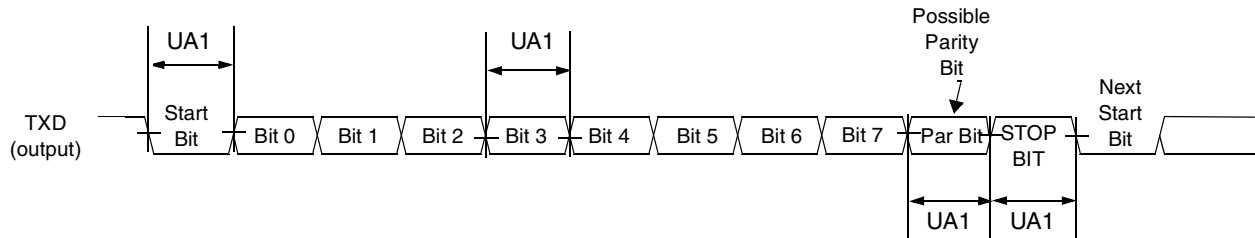
Figure 85. UART RS-232 Serial Mode Transmit Timing Diagram
