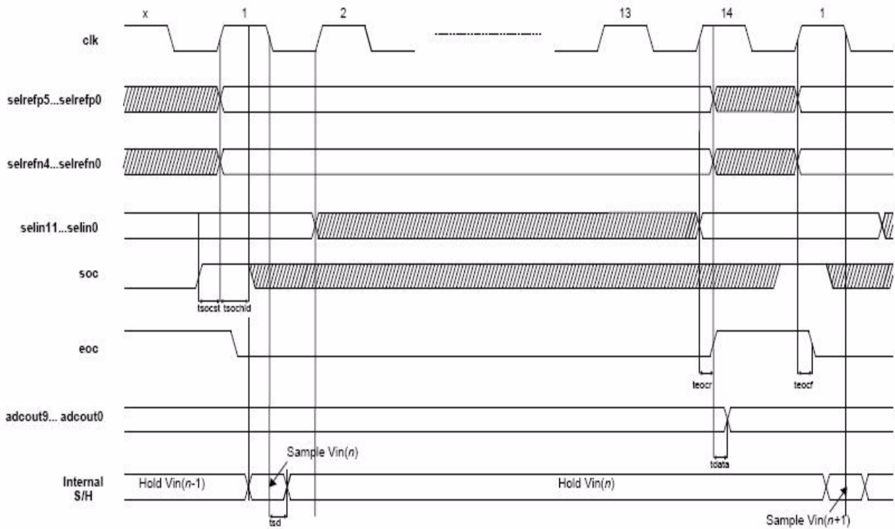
Figure 83. Timing for ADC Normal Operation
