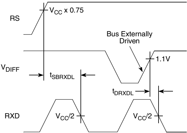
Figure 61. Timing Diagram for FlexCAN Standby Signal
