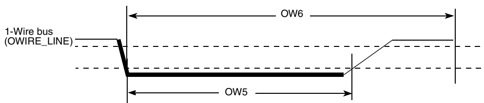
Figure 8. Write 0 Sequence Timing Diagram
