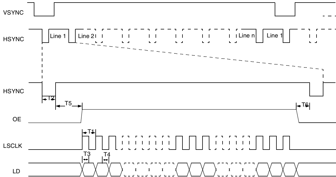
Figure 66. LCDC TFT Mode Timing Diagram
