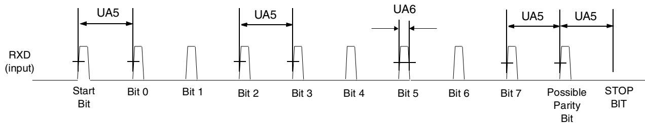
Figure 88. UART IrDA Mode Receive Timing Diagram
