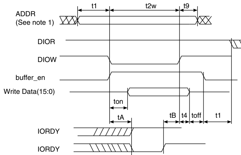
Figure 12. PIO Write Mode Timing
