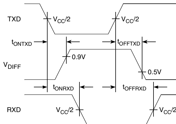
Figure 60. FlexCAN Timing Diagram
