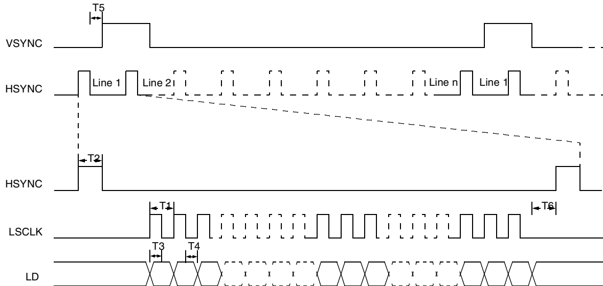
Figure 65. LCDC Non-TFT Mode Timing Diagram
