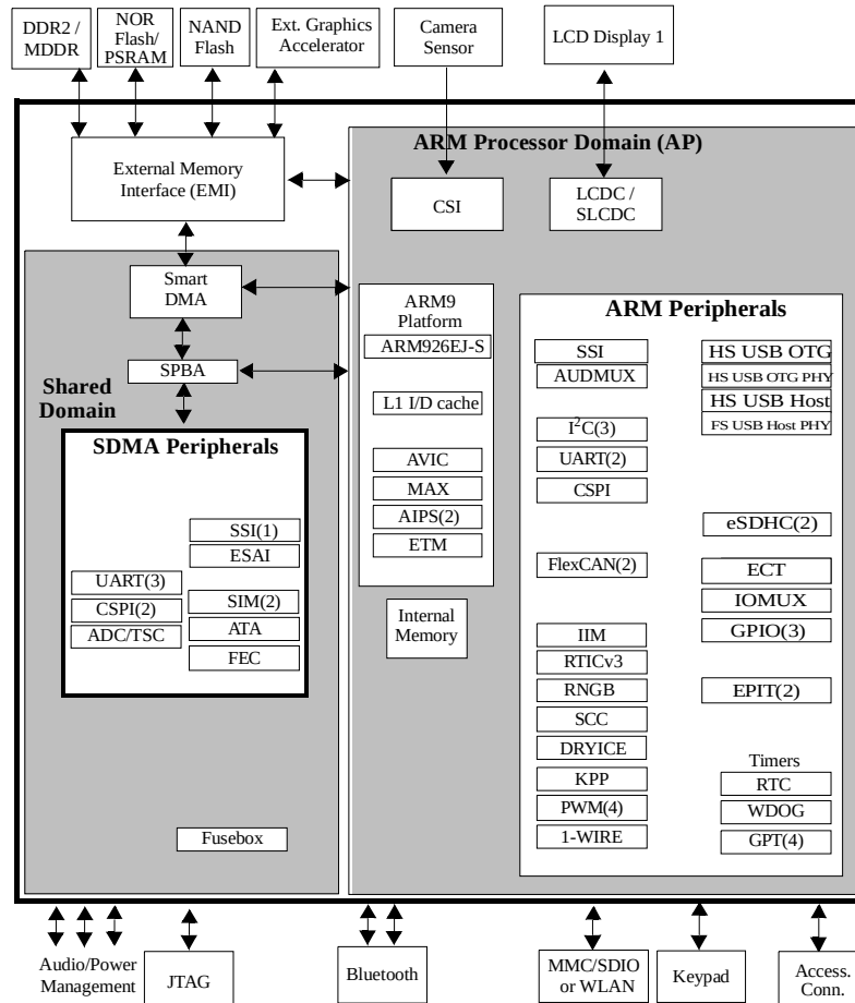
Figure 1. i.MX25 Simplified Interface Block Diagram
