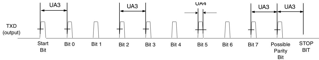
Figure 87. UART IrDA Mode Transmit Timing Diagram
