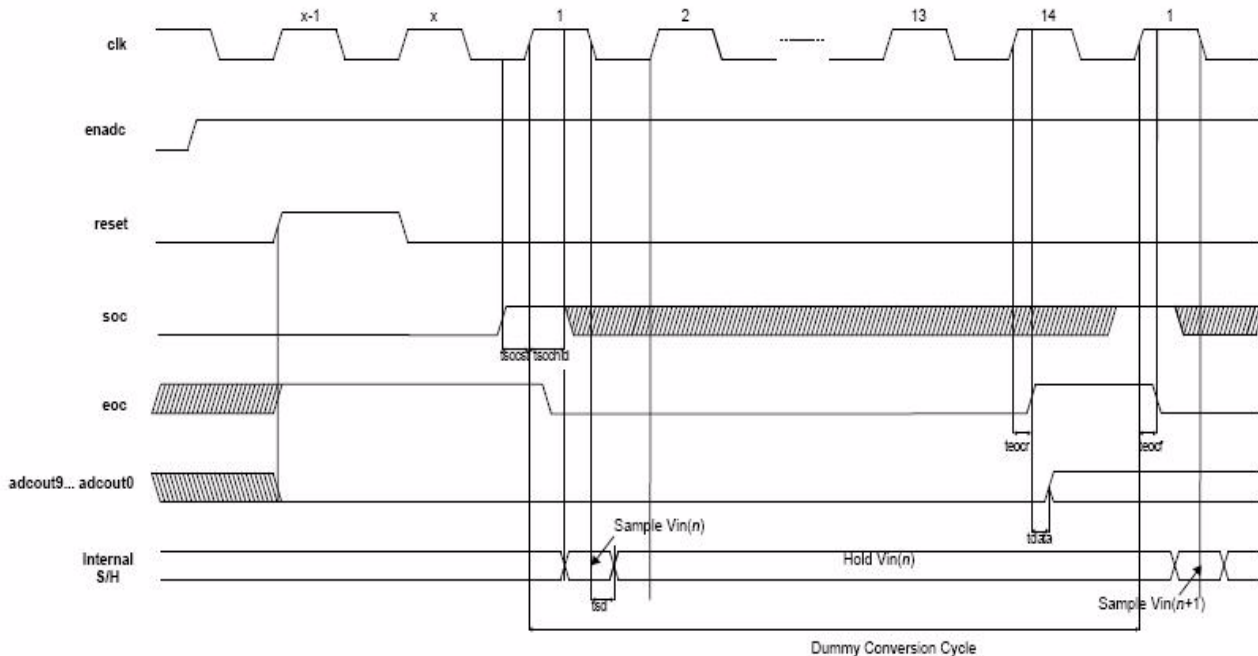
Figure 82. Start-up Sequence
