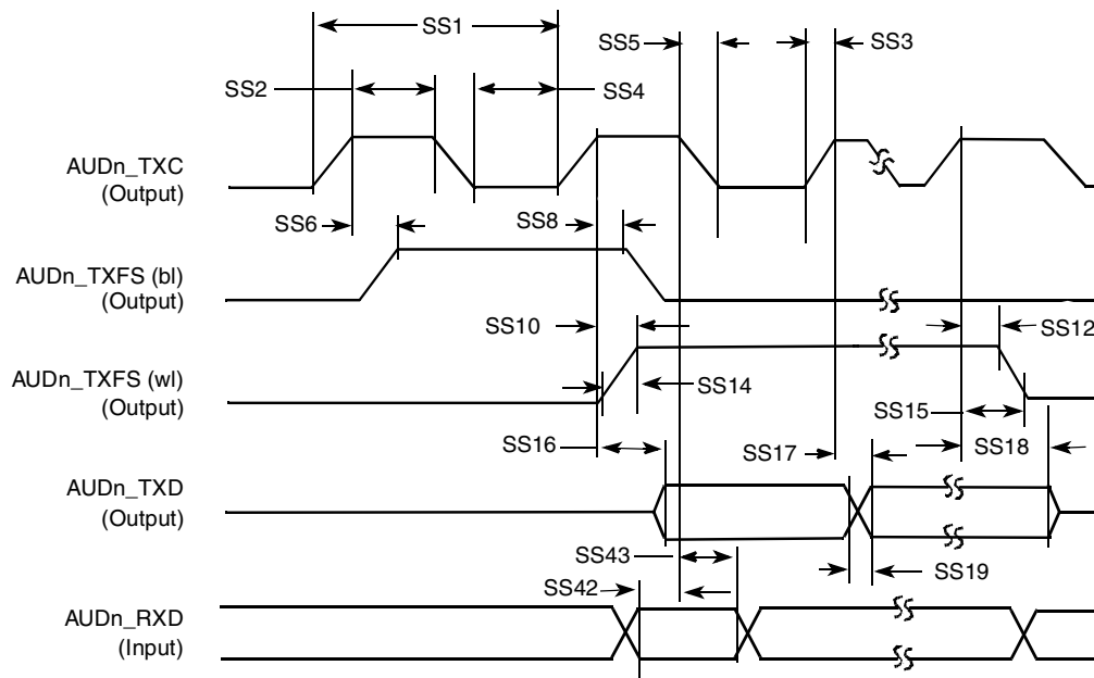
Figure 78. SSI Transmitter with Internal Clock Timing Diagram
