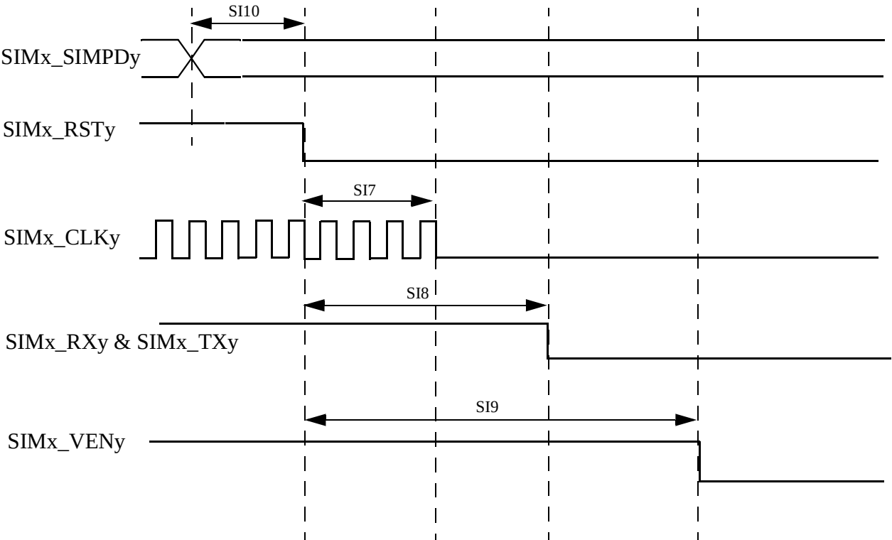
Figure 71. SmartCard Interface Power Down AC Timing
