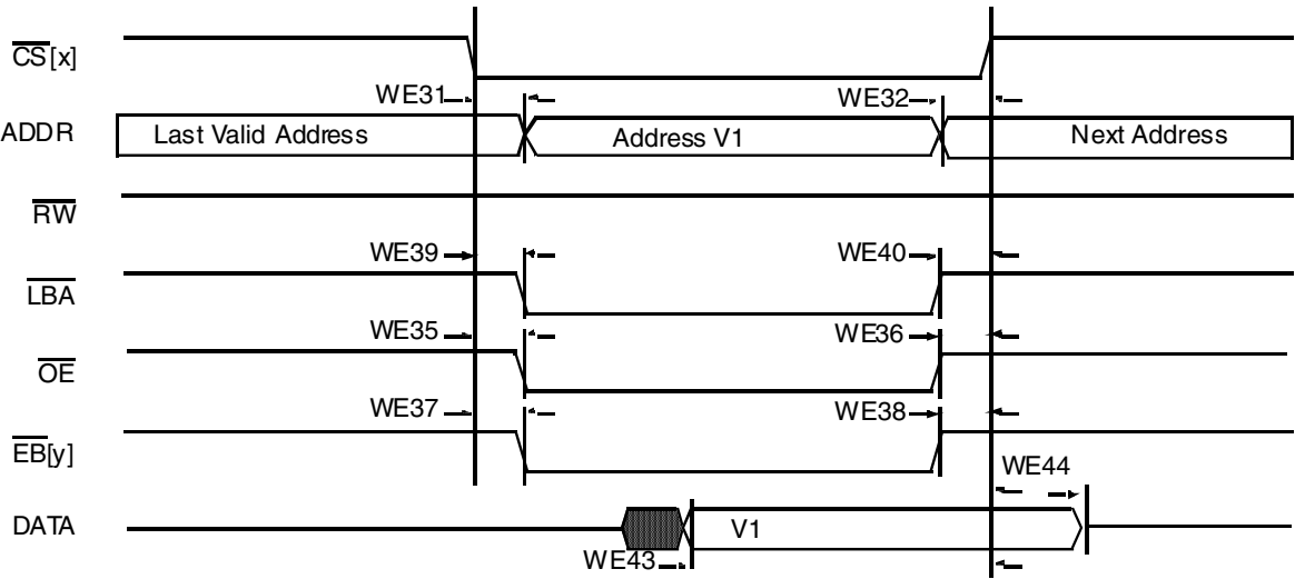
Figure 45. Asynchronous Memory Read Access
