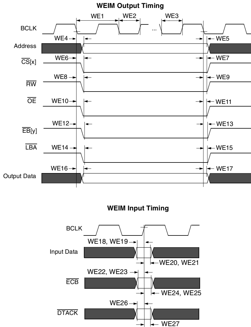
Figure 38. WEIM Bus Timing Diagram
