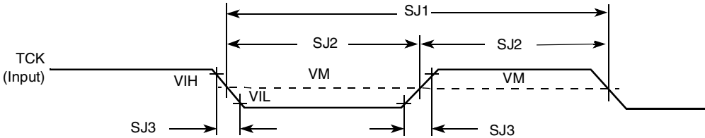
Figure 72. Test Clock Input Timing Diagram
