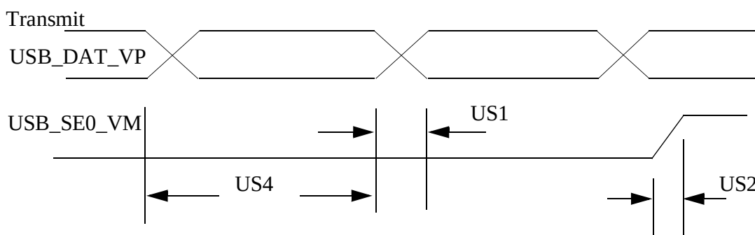
Figure 89. USB Transmit Waveform in DAT_SE0 Bidirectional Mode
