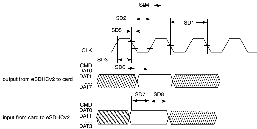
Figure 54. eSDHCv2 Timing
