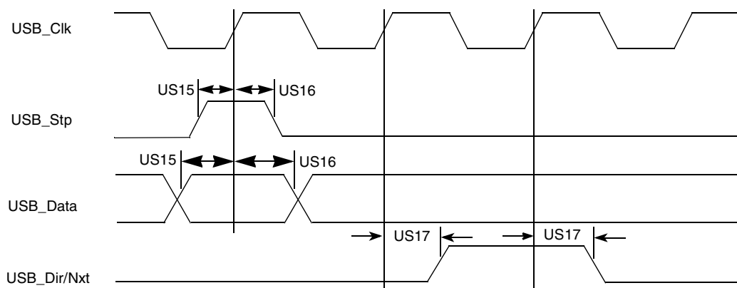
Figure 97. USB Parallel Mode Transmit/Receive Waveform
