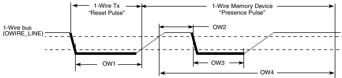
Figure 7. 1-Wire RPP Timing Diagram
