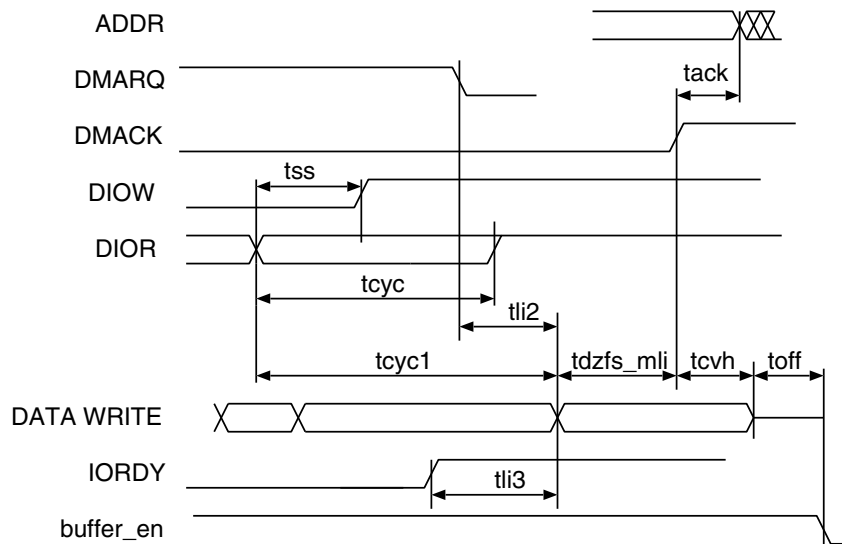
Figure 19. Timing for Host-Terminated UDMA Out-Transfer
