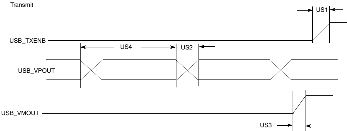
Figure 93. USB Transmit Waveform in VP_VM Bidirectional Mode
