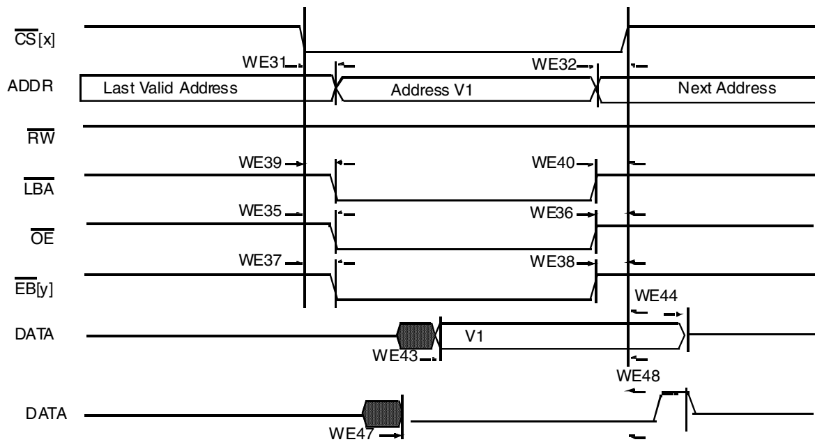
Figure 49. DTACK Read Access
