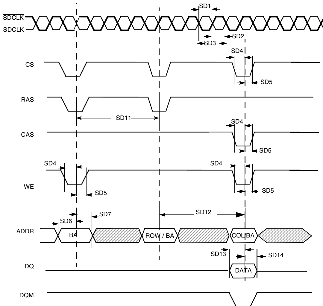
Figure 26. SDR SDRAM Write Cycle Timing Diagram
