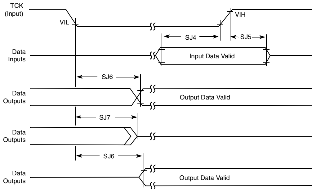
Figure 73. Boundary Scan (JTAG) Timing Diagram
