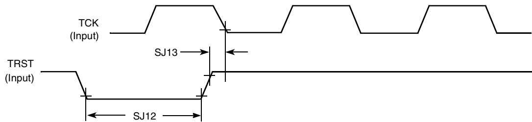
Figure 75. \overline{\text{TRST}} Timing Diagram
