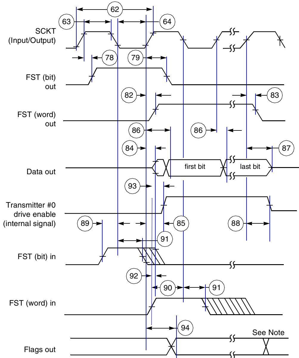
Figure 50. ESAI Transmit Timing
