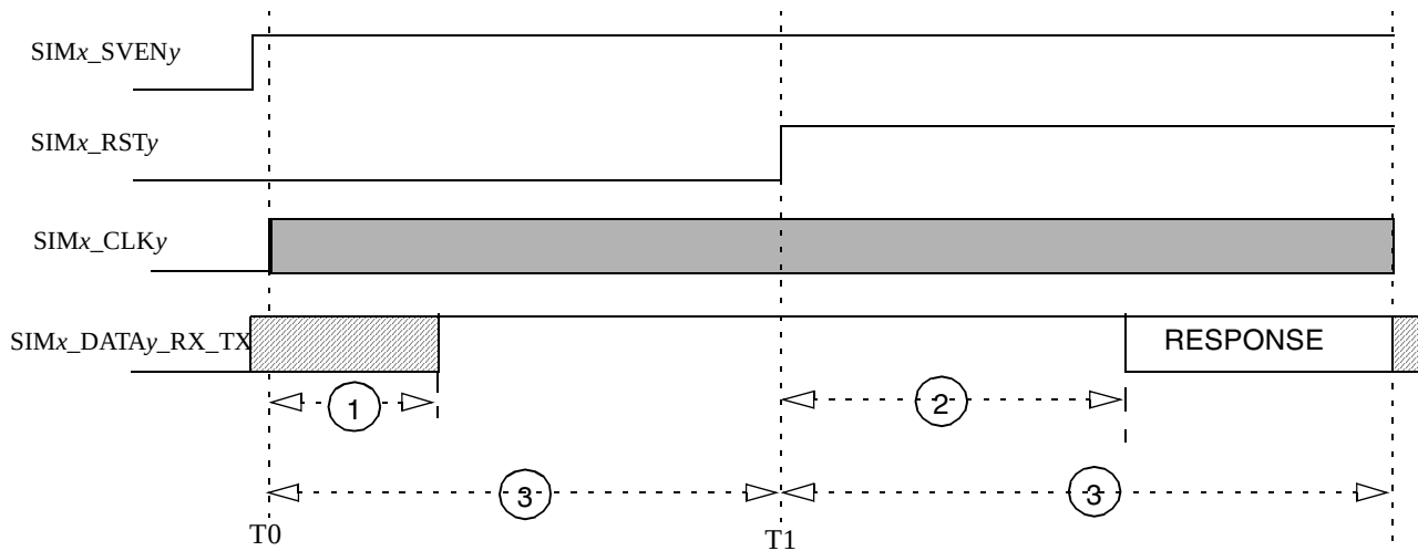
Figure 70. Active-Low-Reset SIM Card Reset Sequence
