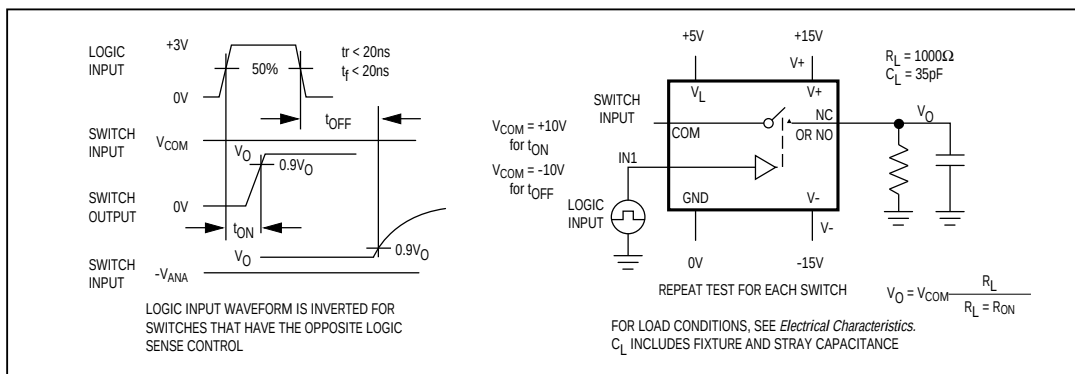
Figure 2. Switching-Time Test Circuit
