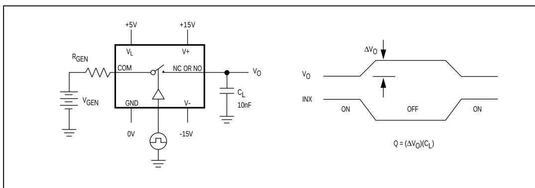
Figure 4. Charge-Injection Test Circuit
