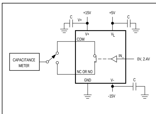
Figure 7. Channel On-Capacitance
