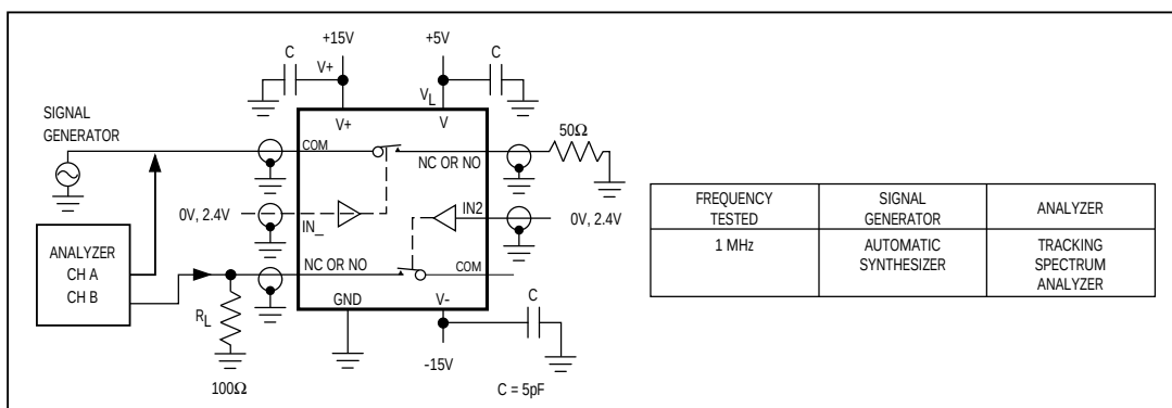
Figure 6. Crosstalk Test Circuit
