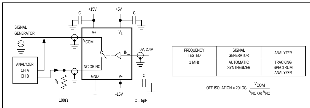
Figure 5. Off Isolation
