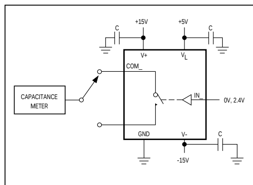
Figure 8. Channel Off-Capacitance
