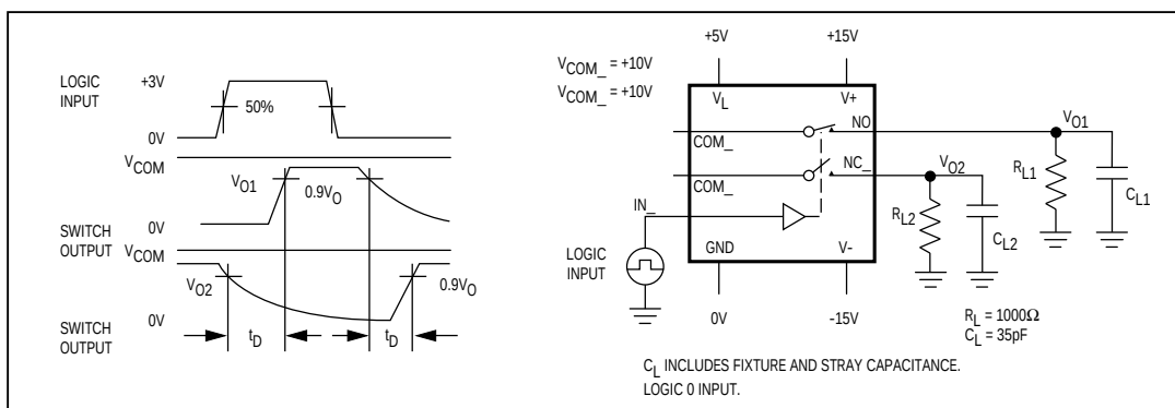
Figure 3. Break-Before-Make Test Circuit
