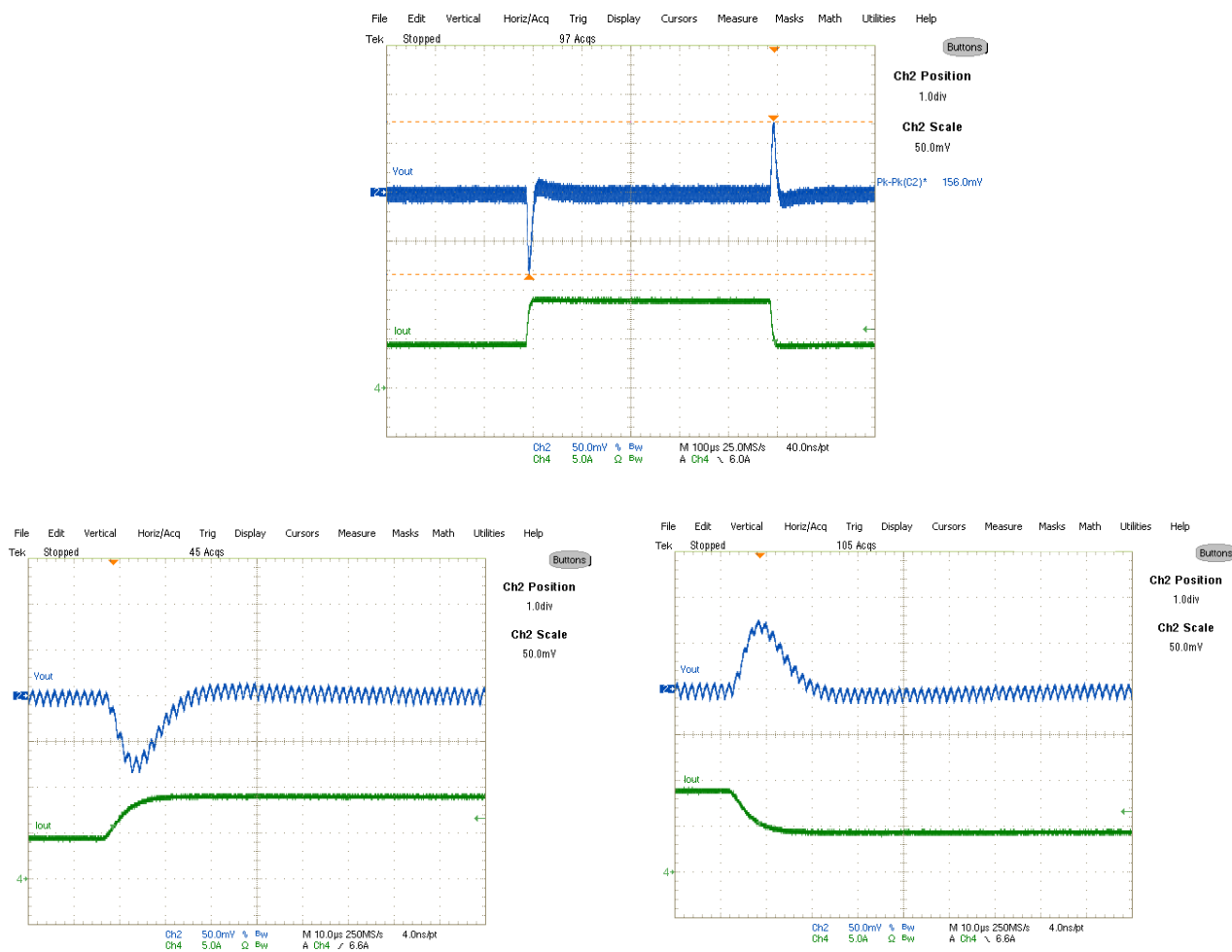
Fig. 24: Transient Response, 4.5A to 9A step 2.5A/μs
