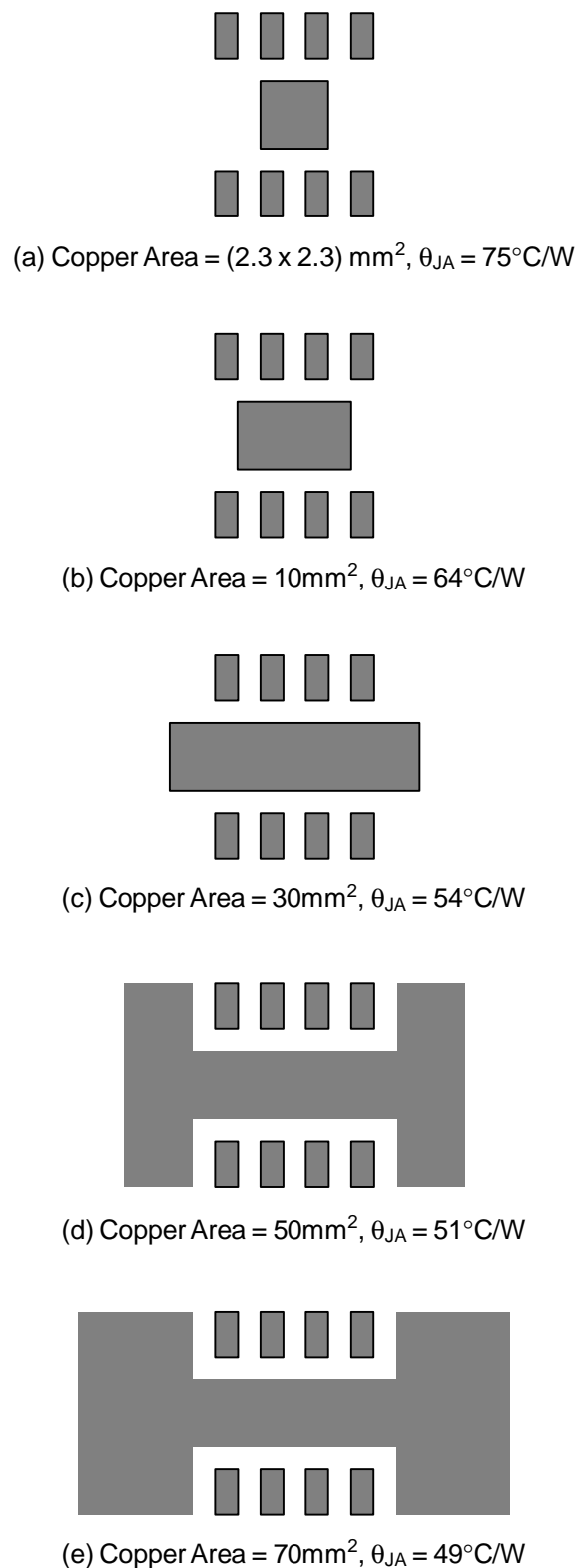
Figure 4. Thermal Resistance vs. Copper Area Layout Thermal Design
