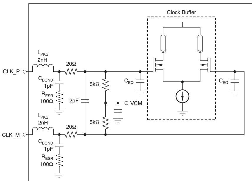
Figure 61. Internal Clock Buffer
