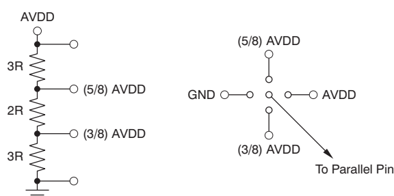
Figure 8. Simple Scheme to Configure the Parallel Pins
