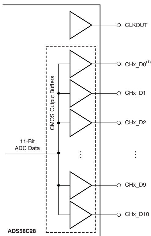
Figure 68. CMOS Interface
