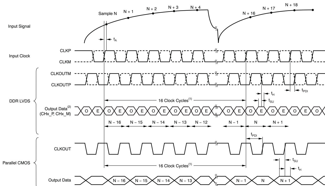
Figure 5. Latency Diagram
