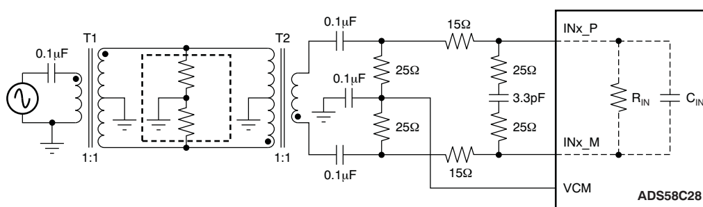
Figure 57. Drive Circuit with Low Bandwidth (for Low Input Frequencies)
