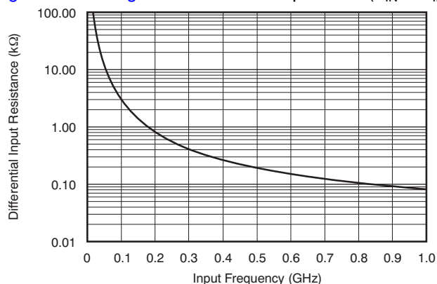
Figure 55. ADC Analog Input Resistance ( R_{IN} ) Across Frequency
