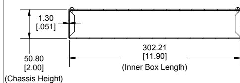
Bottom Plate (Sold Separately)
