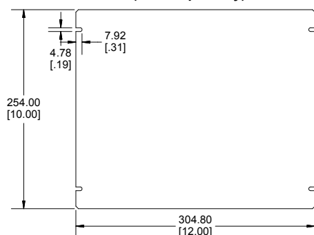
Bottom Plate (Sold Separately)
