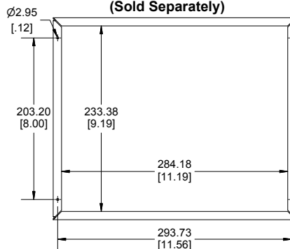
Bottom View of Chassis (Sold Separately)
