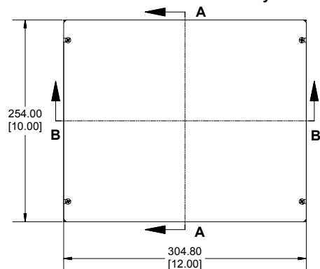
Bottom View of Assembly
