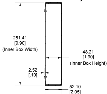
Bottom View of Chassis (Sold Separately)
