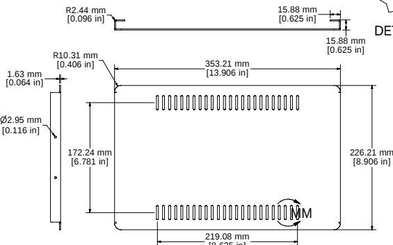
REAR PANEL - VIEW FROM OUTSIDE
