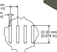
DETAIL MM
