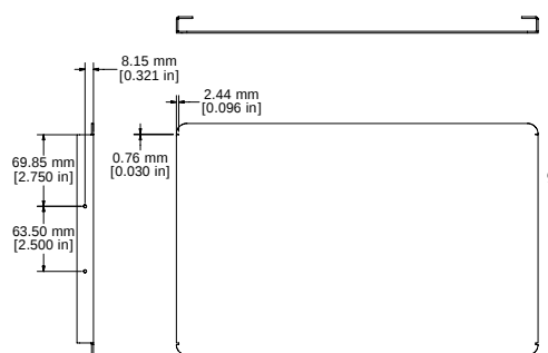
FRONT PANEL - VIEW FROM OUTSIDE
