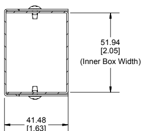
SECTION A-A End View of Assembly
