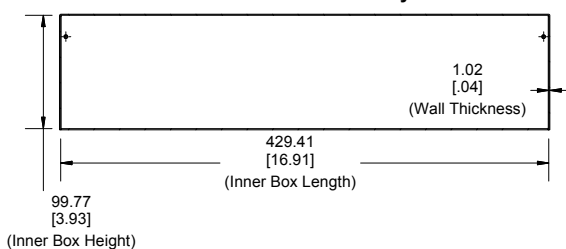
SECTION B-B Side View of Assembly
