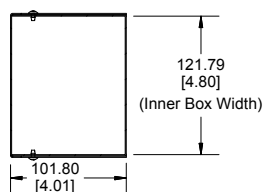
SECTION A-A End View of Assembly
