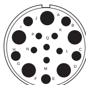
36-14 6 #16(K-N,P,Q) 5 #12(B,D,F,H,J) 5 #8(A,C,E,G,I)
