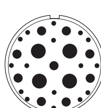
40-10 16 #16(A,B,E-H,M,N,P Q,V-Y,b,c) 9 #8(C,D,I,L,O,R,U,Z,a) 4 #4(K,J,S,T)
