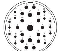
36-9 14 #16(A-G,Z-f) 14 #12(H-N,S-Y) 2 #8(O,R) 1 #4(P)
