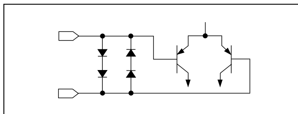
Figure 1. Input Protection Circuit
