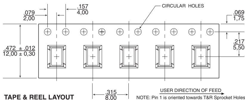
TAPE & REEL LAYOUT
