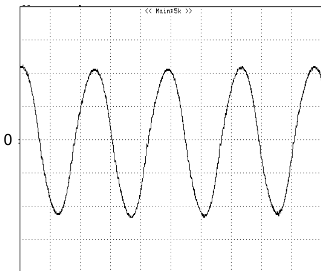
Figure 11: Input Terminal Ripple Current, i_c , at full rated output current and nominal input voltage with 12\mu H source impedance and 33\mu F electrolytic capacitor (50 mA/div, 1μs/div)
