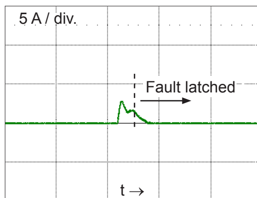
Figure 4: Short-to-Ground Event
