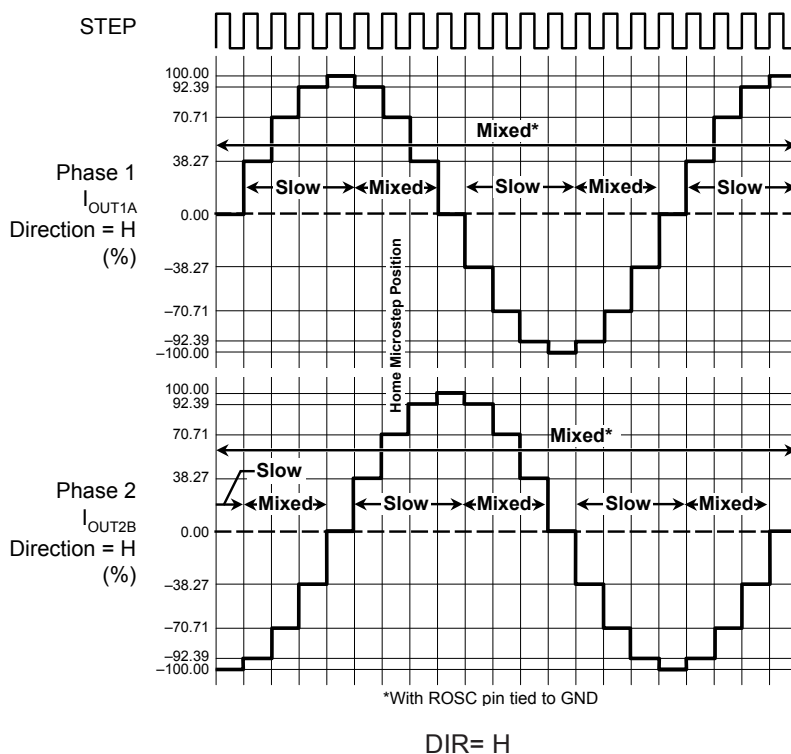
Figure 12: Decay Modes for Quarter-Step Increments
