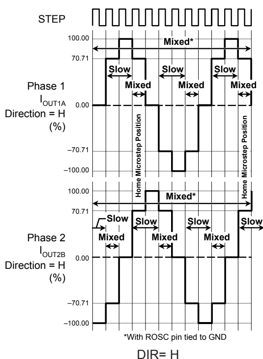
Figure 11: Decay Modes for Half-Step Increments
