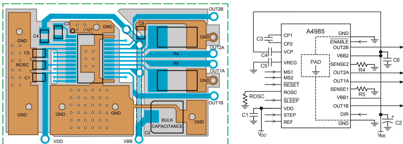
Figure 9: LP Package Typical Application and Circuit Layout
