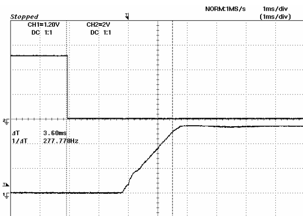
Figure 17: Turn on delay time at remote turn on with external capacitors (Co= 3000 μF) 5Vin, 3.3V/6A out
