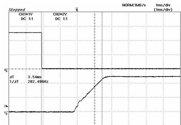
Figure 18: Turn on delay time at remote turn on with external capacitors (Co= 3000 μF) 3.3Vin, 2.5V/6A out
