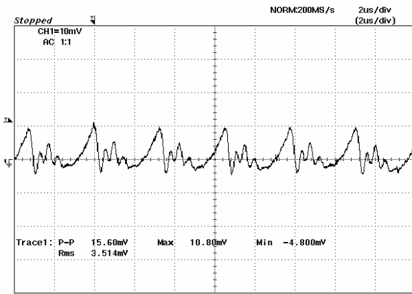
Figure 7: Output ripple & noise at 3.3Vin, 2.5V/6A out
