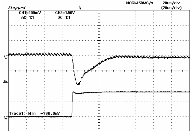
Figure 24: Typical transient response to step load change at 2.5A/\mu s from 50% to 100% of I_o , max at 3.3V_{in} , 2.5V_{out} ( C_{out} = 1\mu F ceramic, 10\mu F tantalum)
