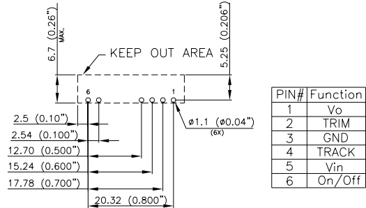
RECOMMENDED PWB PAD LAYOUT
