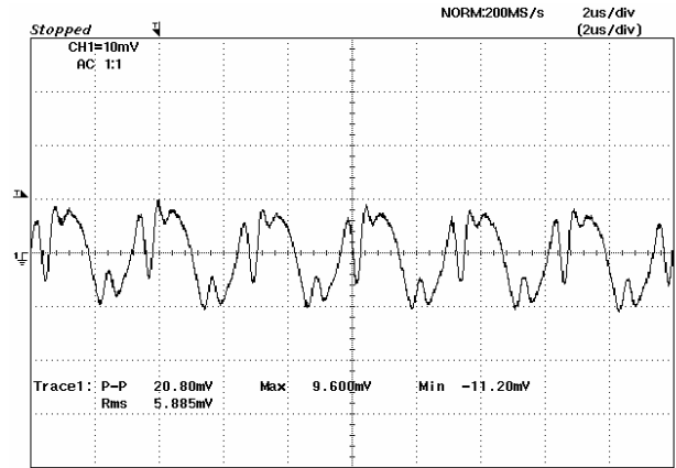
Figure 8: Output ripple & noise at 3.3Vin, 1.8V/6A out
