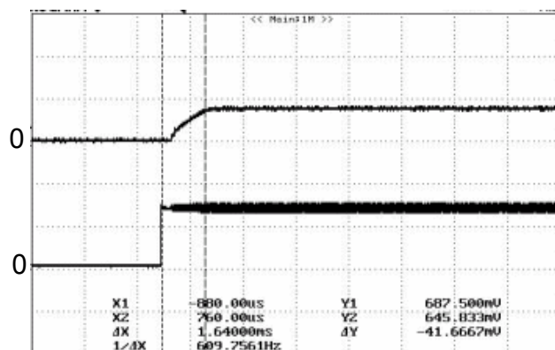
Figure 14: Turn on delay time Remote On/Off, 1.5V/6A out Ch1: Enable Ch4: Vout
