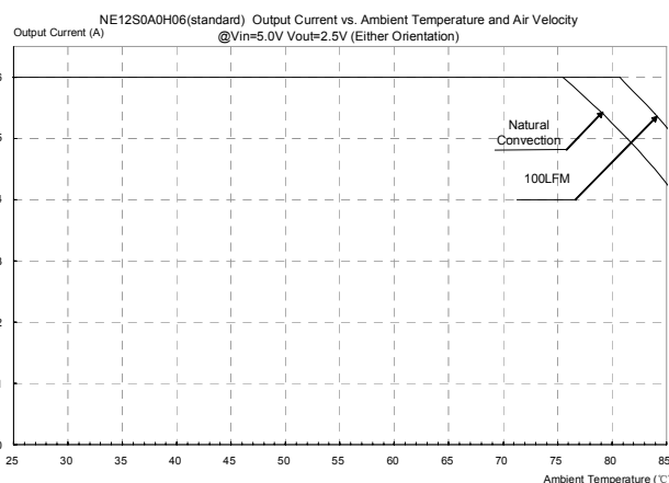
Figure 39: Output current vs. ambient temperature and air velocity @ Vin =5V, Vout=2.5V (Either Orientation)
