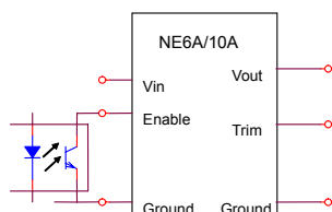
Figure 19: Enable Input drive circuit for NE series
