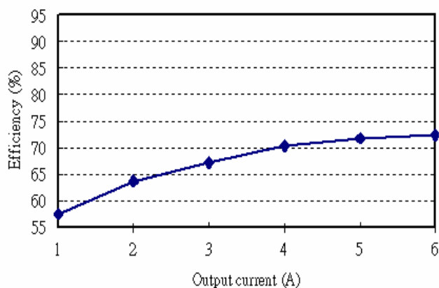
Figure 1: Converter efficiency vs. output current (0.59V output voltage, 12V input voltage)
