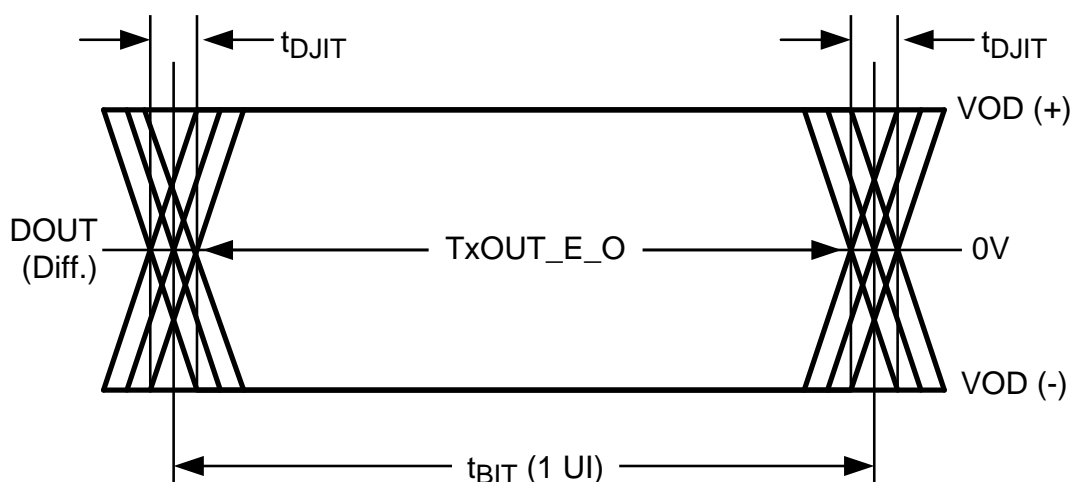
Figure 14. DS92LV0411 Output Jitter
