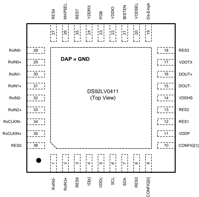
Figure 1. DS92LV0411 — Top View
