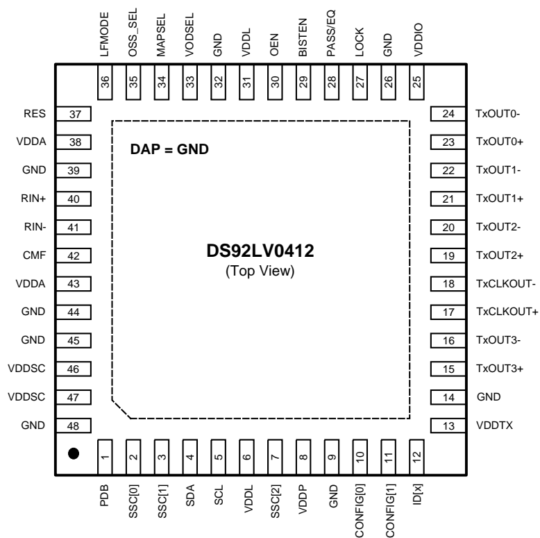
Figure 2. DS92LV0412 — Top View
