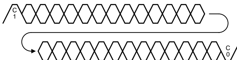
Figure 21. Channel Link II Serial Stream
