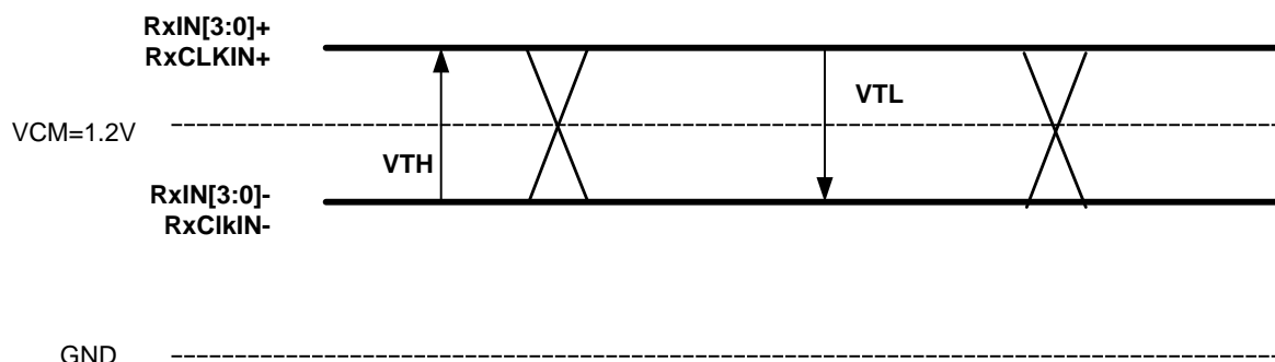
Figure 3. Channel Link DC VTH/VTL Definition
