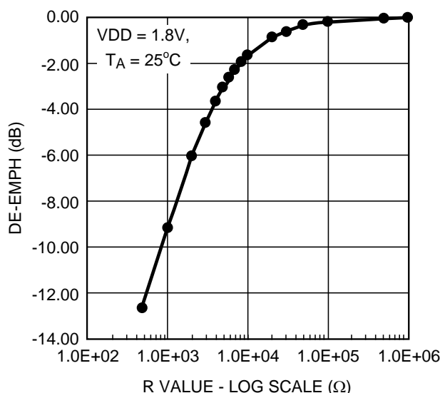
Figure 25. De-Emph vs. R value
