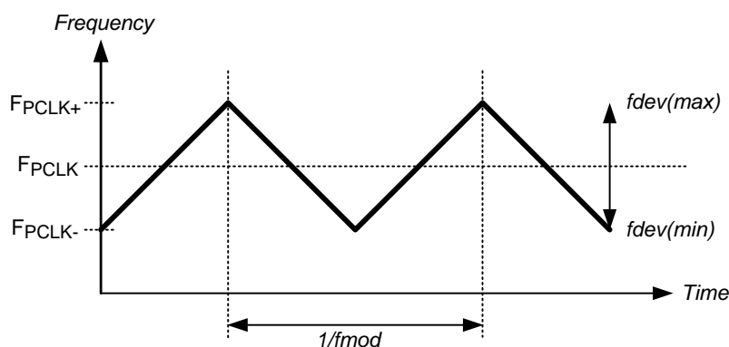
Figure 26. SSCG Waveform
