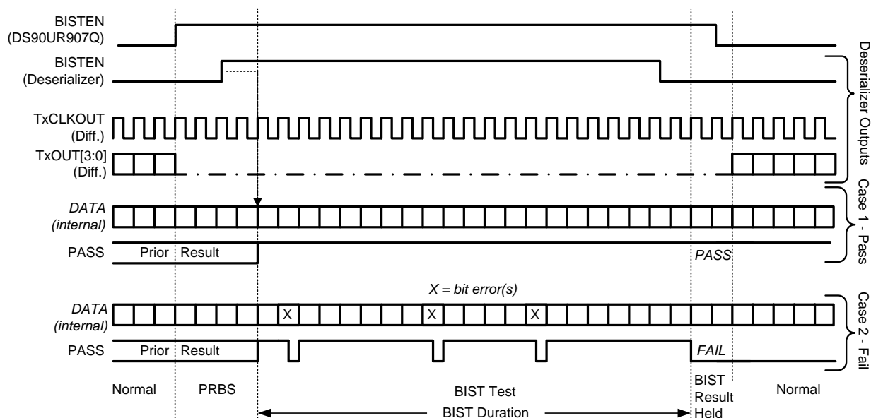
Figure 28. BIST Waveforms
