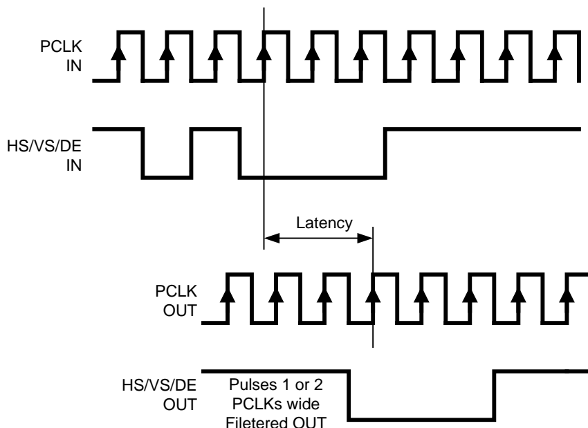
Figure 24. Video Control Signal Filter Waveform
