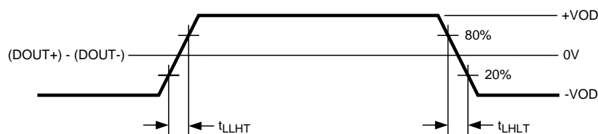
Figure 6. DS92LV0411 Output Transition Times
