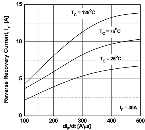
Figure 7. Typical Reverse Recovery Current vs. di_F/dt
