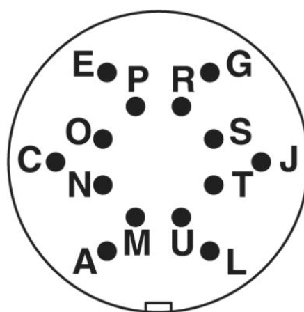
M16 plug connection pin, 14-pos.
