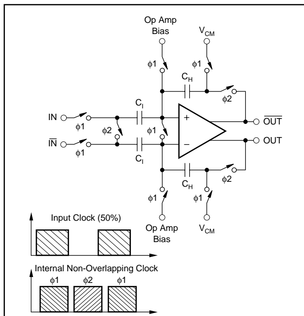
FIGURE 1. Input Track-and-Hold Configuration with Timing Signals.
